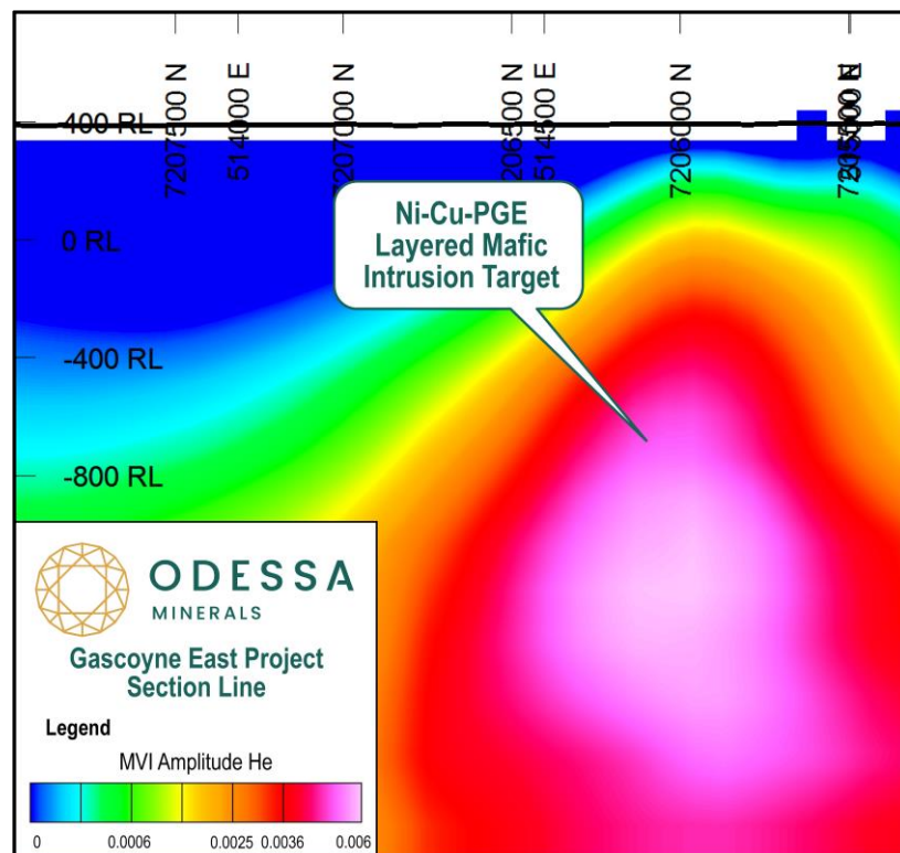
Figure 3: MVI Amplitude Section through the interpreted layered mafic intrusion target.
