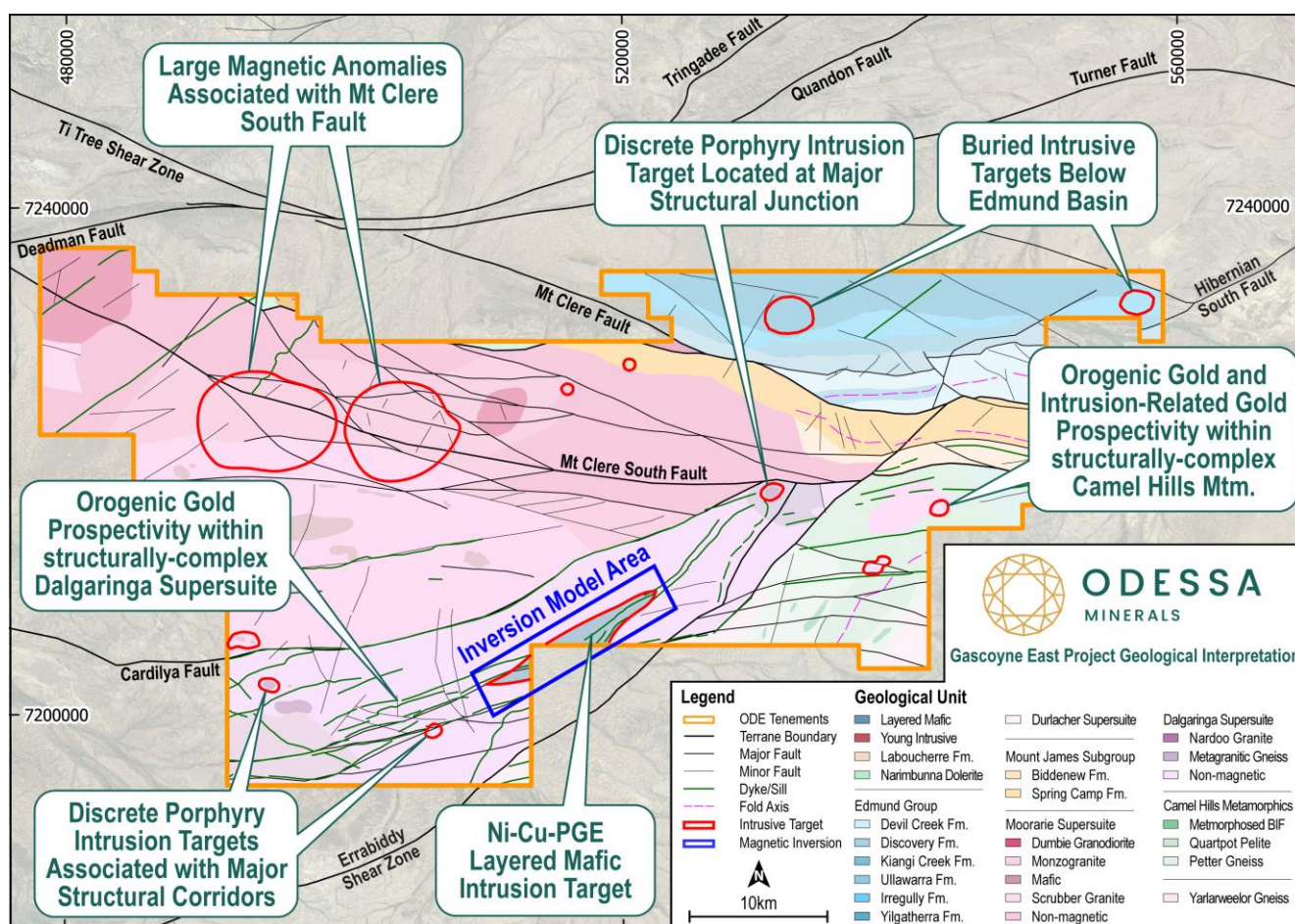
Figure 1: Interpreted bedrock geology with key intrusion targets outlined. Modelled magnetic inversion area displayed.
