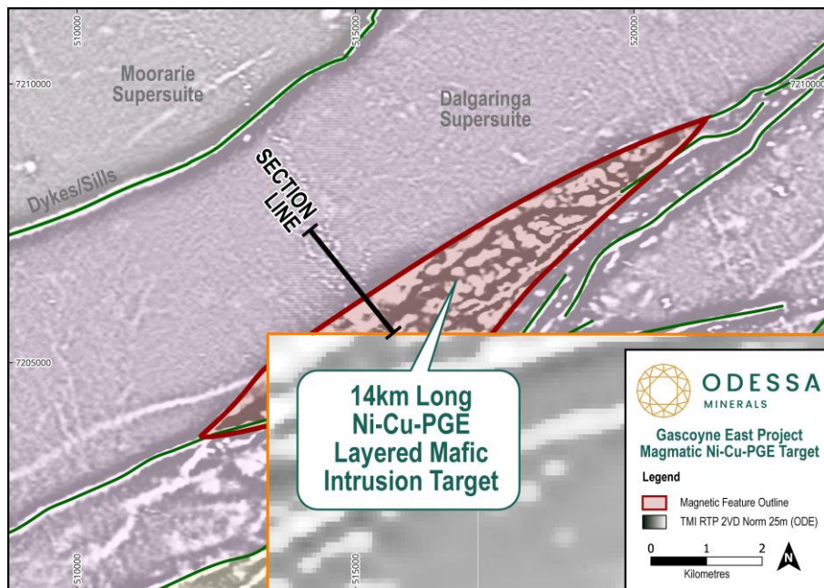
Figure 2: Geological map showing inversion section line through the interpreted layered mafic intrusion underlain by magnetic imagery.
