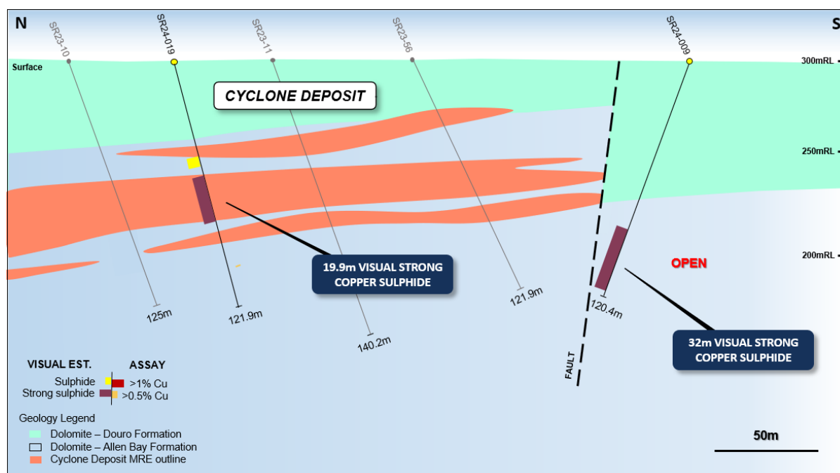
Figure 6: Geological section view at 464,650E showing the visual results for drill holes SR24-009 and SR24-019, and the existing Cyclone Deposit resource outline.
