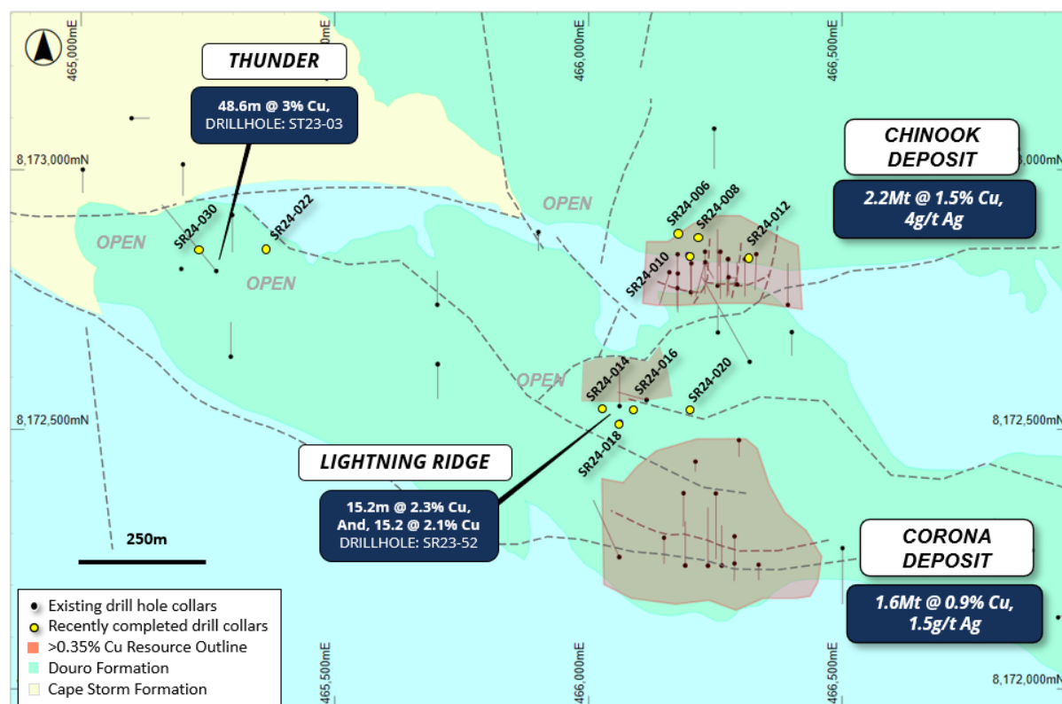
Figure 3: Plan view of the Chinook, Corona, Thunder, and Lightning Ridge areas showing the known copper deposits and interpreted footprint (defined by drilling, MLEM and VTEM) of the near-surface copper mineralisation and drilling overlaying regional geology.
