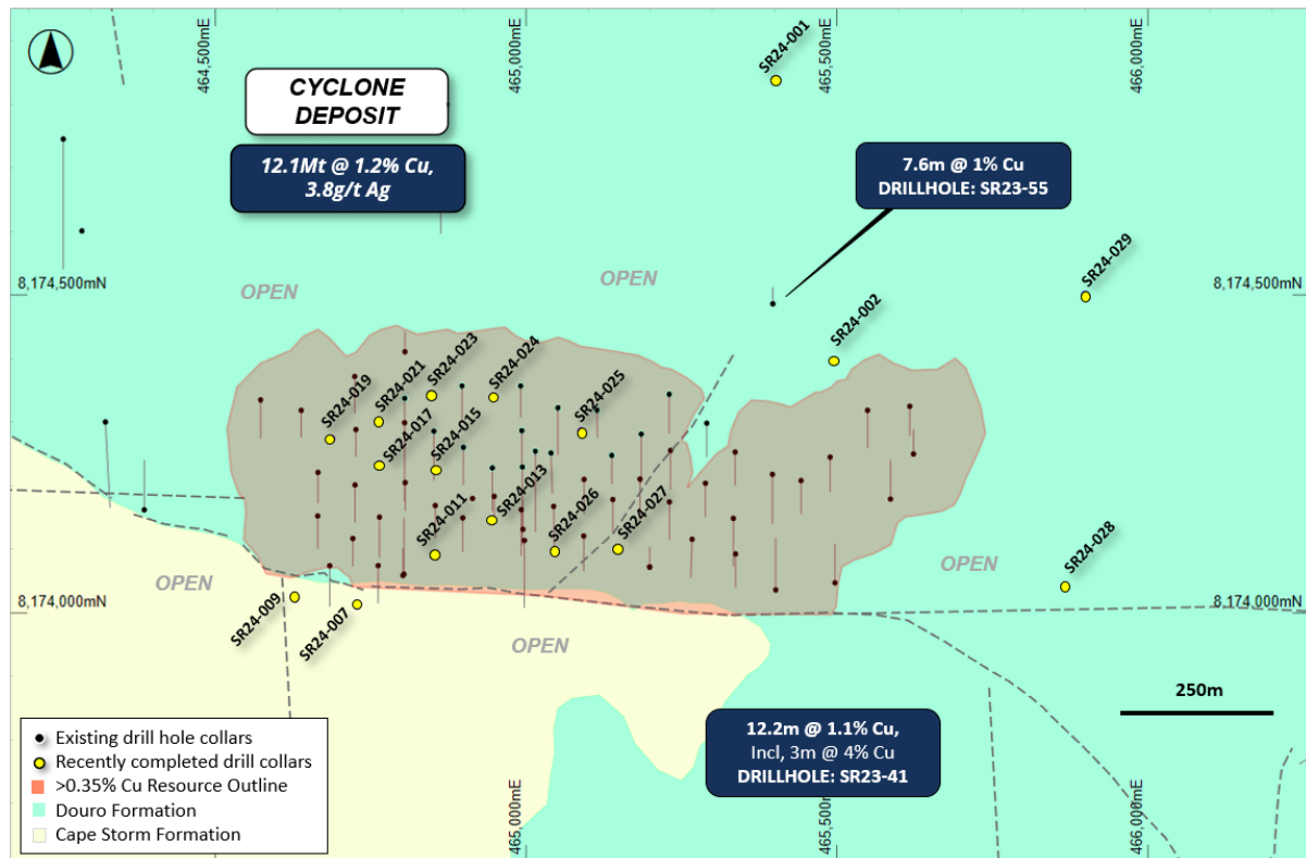
Figure 5: Plan view of the Cyclone Deposit showing the >0.35% Cu resource outline, historical and recent drilling, overlaying regional geology.
