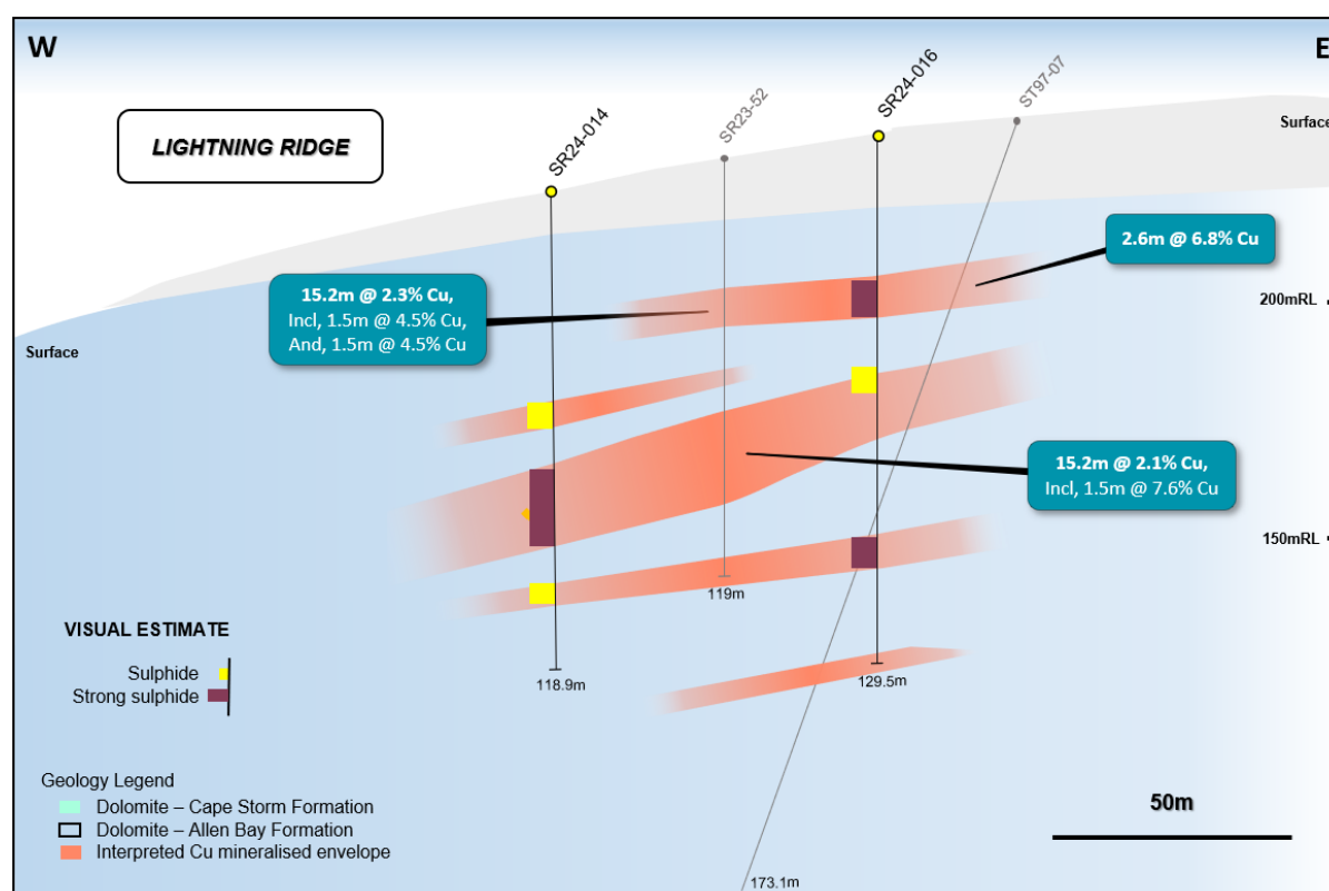
Figure 4: Geological long-section view (looking north) at 8,172,580N showing the visual results for drill holes SR24-14 and SR24-16, historical drilling, and the interpreted copper horizons. Drill hole SR24-18 is located to the south of this section and is therefore not shown.
