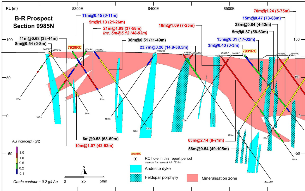
Figure 7: Significant gold intercepts 20 in section 9985N 21 , B-R prospect.
