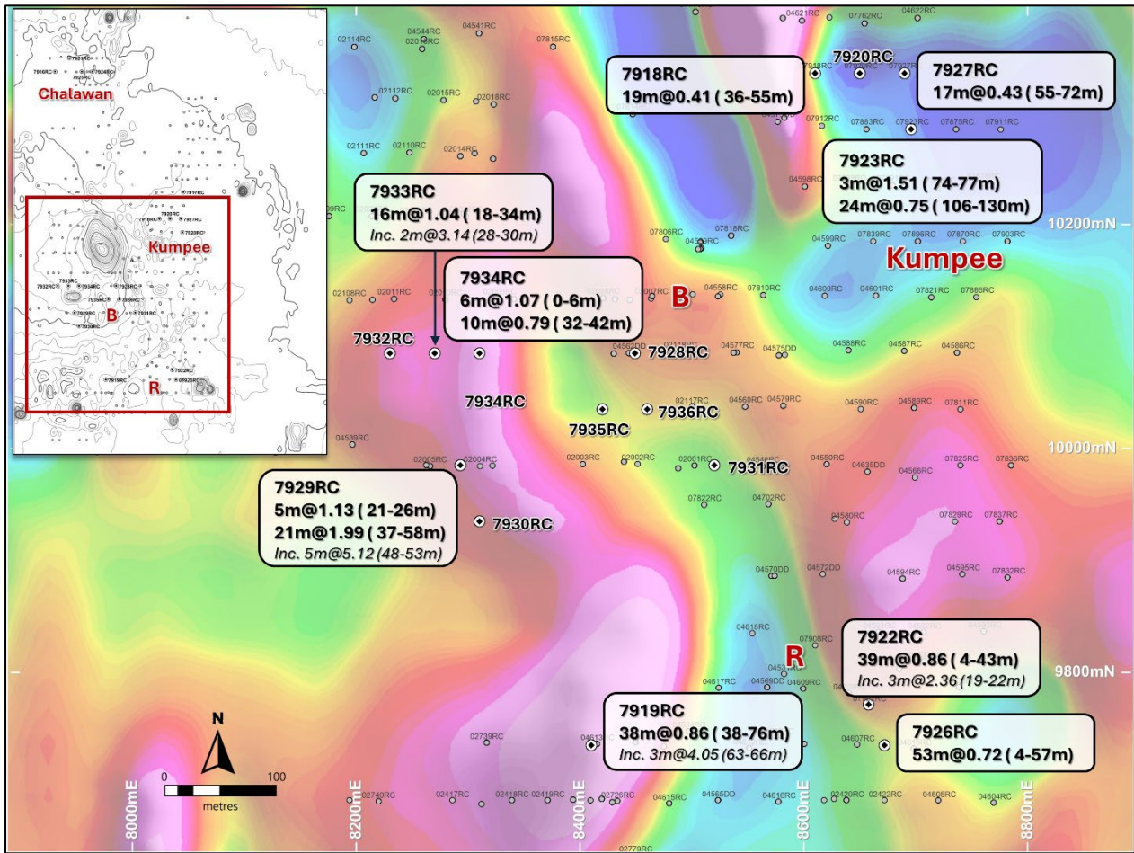
Figure 4: Drill hole locations and gold assay highlights at B-R and Kumpee prospects, overlying IP-chargeability at 50m depth. 13
