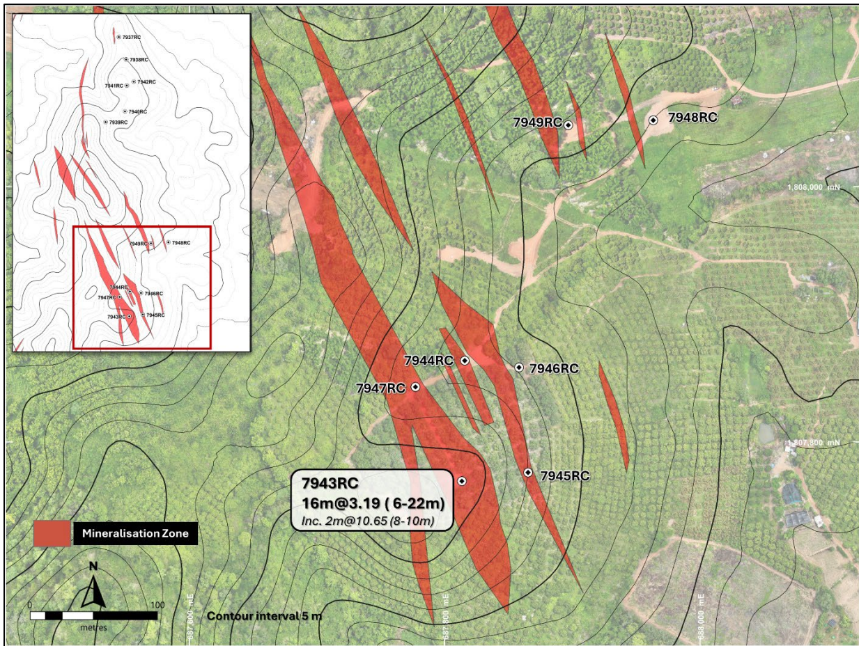
Figure 8: Drill hole locations and gold assay highlights at Nok Kaeo prospect 24 (NKK).
