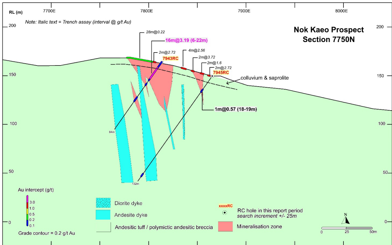
Figure 9: Significant gold intercepts 25 in section 7750N 26 , Nok Kaeo prospect.
