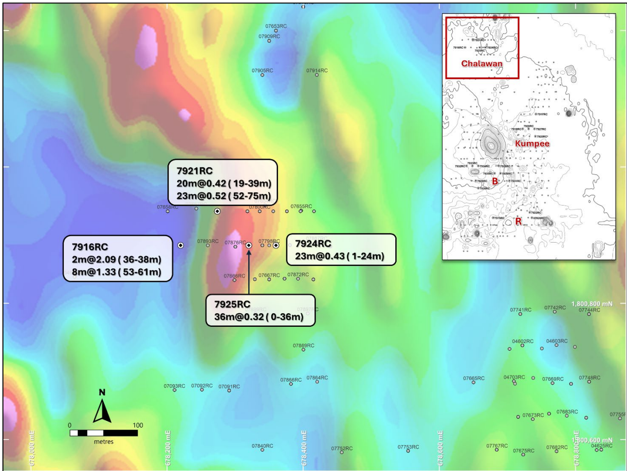
Figure 2: Drill hole locations and gold assay highlights at Chalawan prospect (CLW), overlying IP-resistivity at 50m depth 8 .
