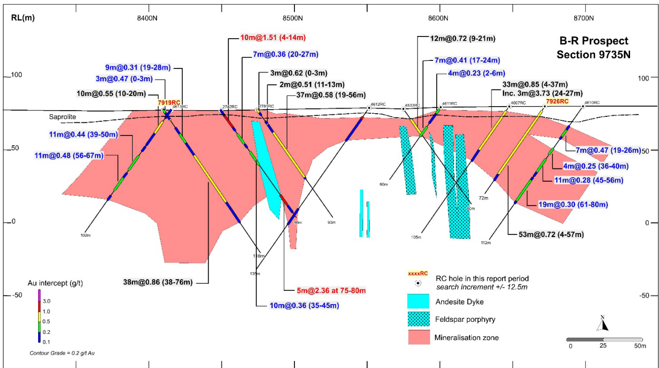
Figure 6: Significant gold intercepts 18 in section 9735N 19 , B-R prospect.
