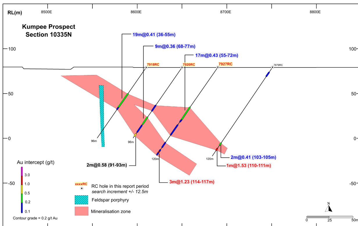
Figure 5: Significant gold intercepts 14 in section 10335N, Kumpee prospect. 15
