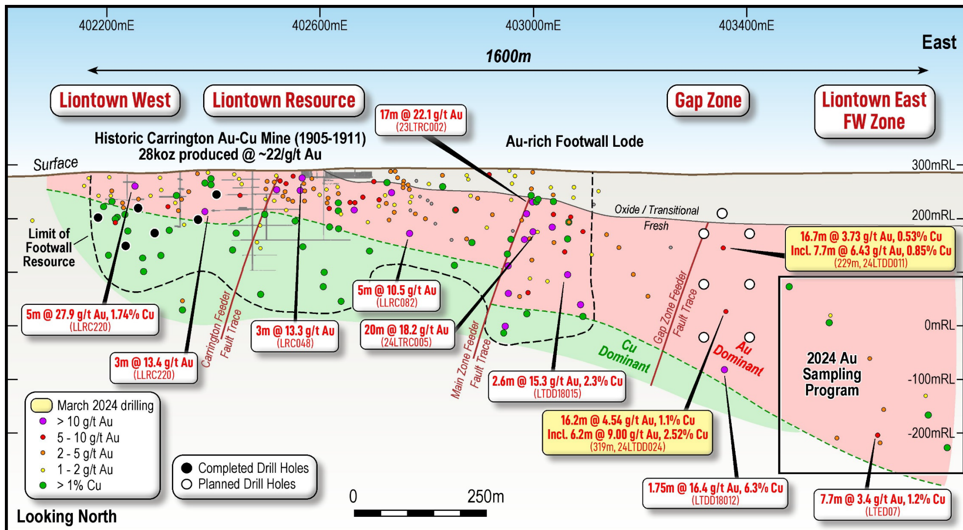
Figure 2: Long section (50m thick) of the ~1,600m long Au-Cu rich footwall horizon extending from the historic Carrington Au-Cu Mine (Lontown Resource), through the recently drilled Au-rich Footwall Lode, the Gap Zone and Lontown East. Completed RC holes are shown (black dots). Planned Resource extension diamond drill holes are shown (white dots). Previously unsampled historic drilling is being sampled in the Au-Cu prospective Lontown East footwall (black box).
