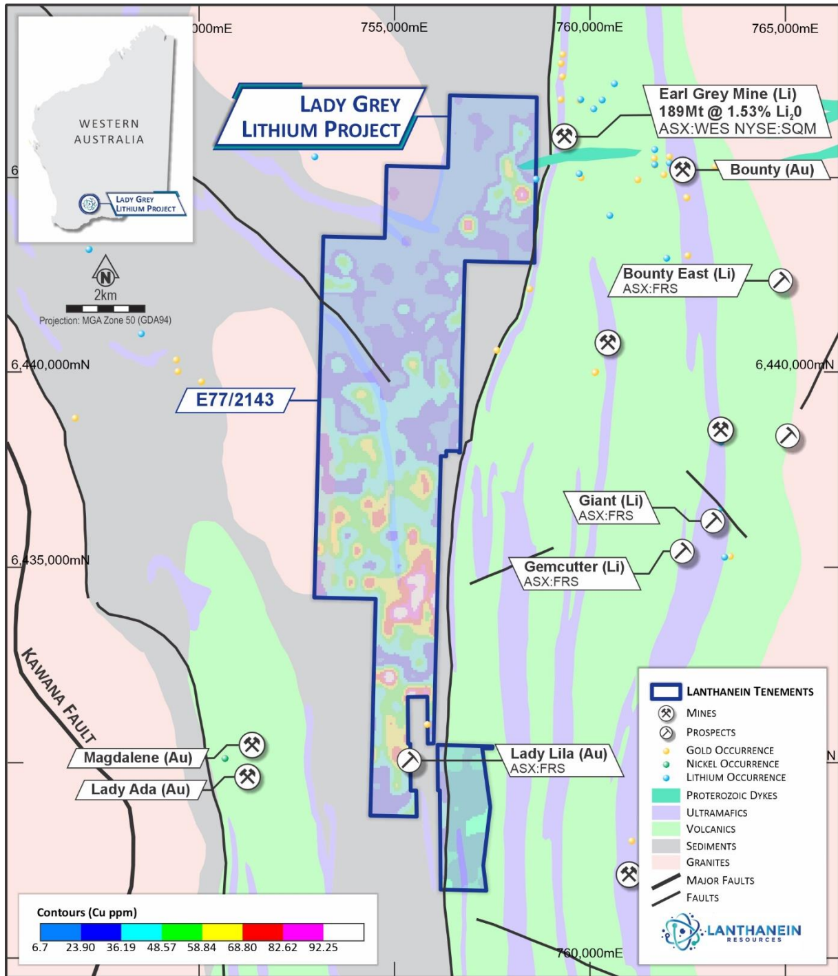
Figure 2: Copper Anomalies at the Lady Grey Lithium Project (refer ASX release 29 April 2024).
