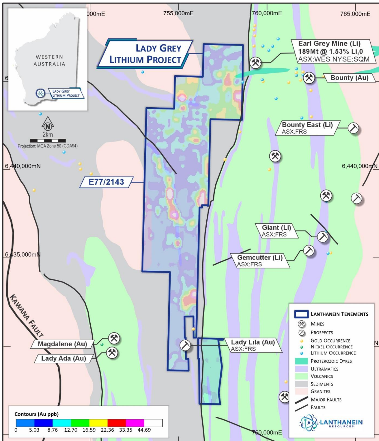
Figure 1: Gold Anomalies at the Lady Grey Lithium Project (refer ASX release 22 April 2024).
