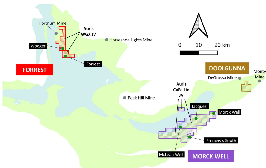
Figure 1: Auris' copper-gold exploration tenement portfolio, with Westgold (WGX) and CuFe Ltd JV areas indicated (as of 30 June 2024)
