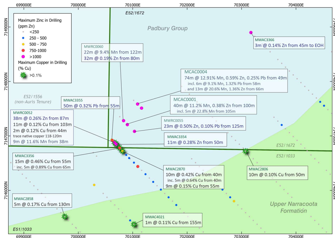
Figure 3: Historical Drilling –Maximum Zn in Drilling, McLean Well Prospect
