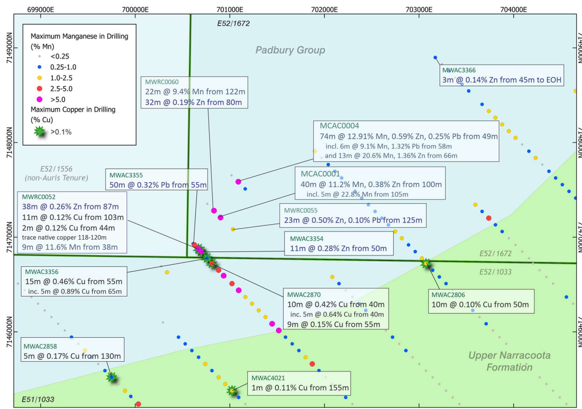
Figure 2: Historical Drilling – Maximum Mn in Drilling, McLean Well Prospect
