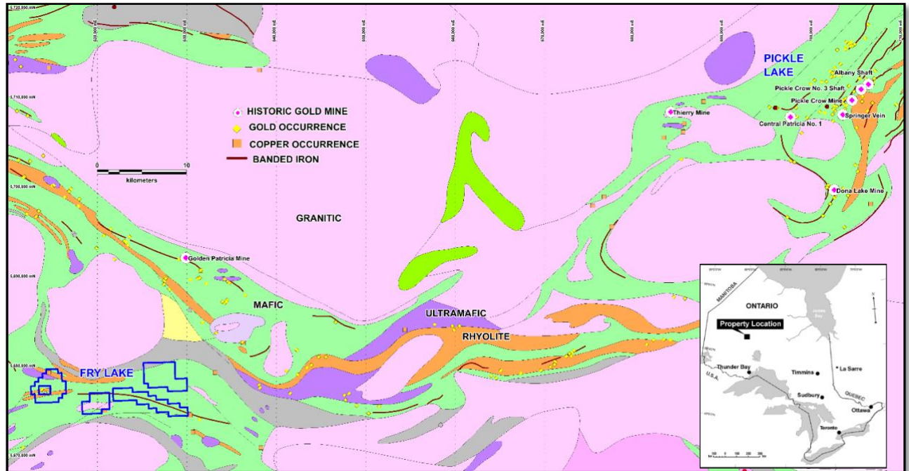
Figure 2: Fry Lake Project in relation to the Pickle Lake and Golden Patricia gold fields and basement geology. Datum UTM NAD83 zone 15.
