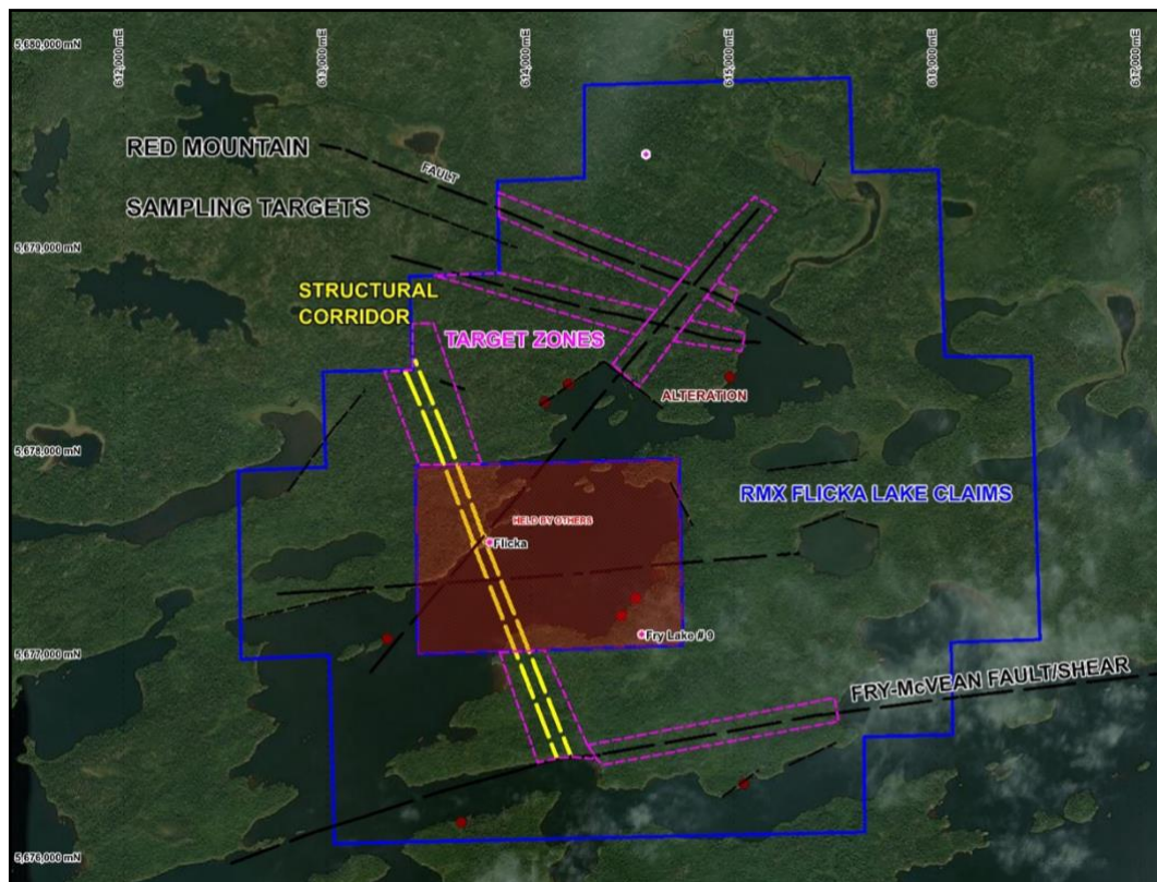
Figure 1: Flicka Lake target areas shown in pink with structural targets, faults, shears, alteration and prospects held by others. Datum UTM NAD83 zone 15
