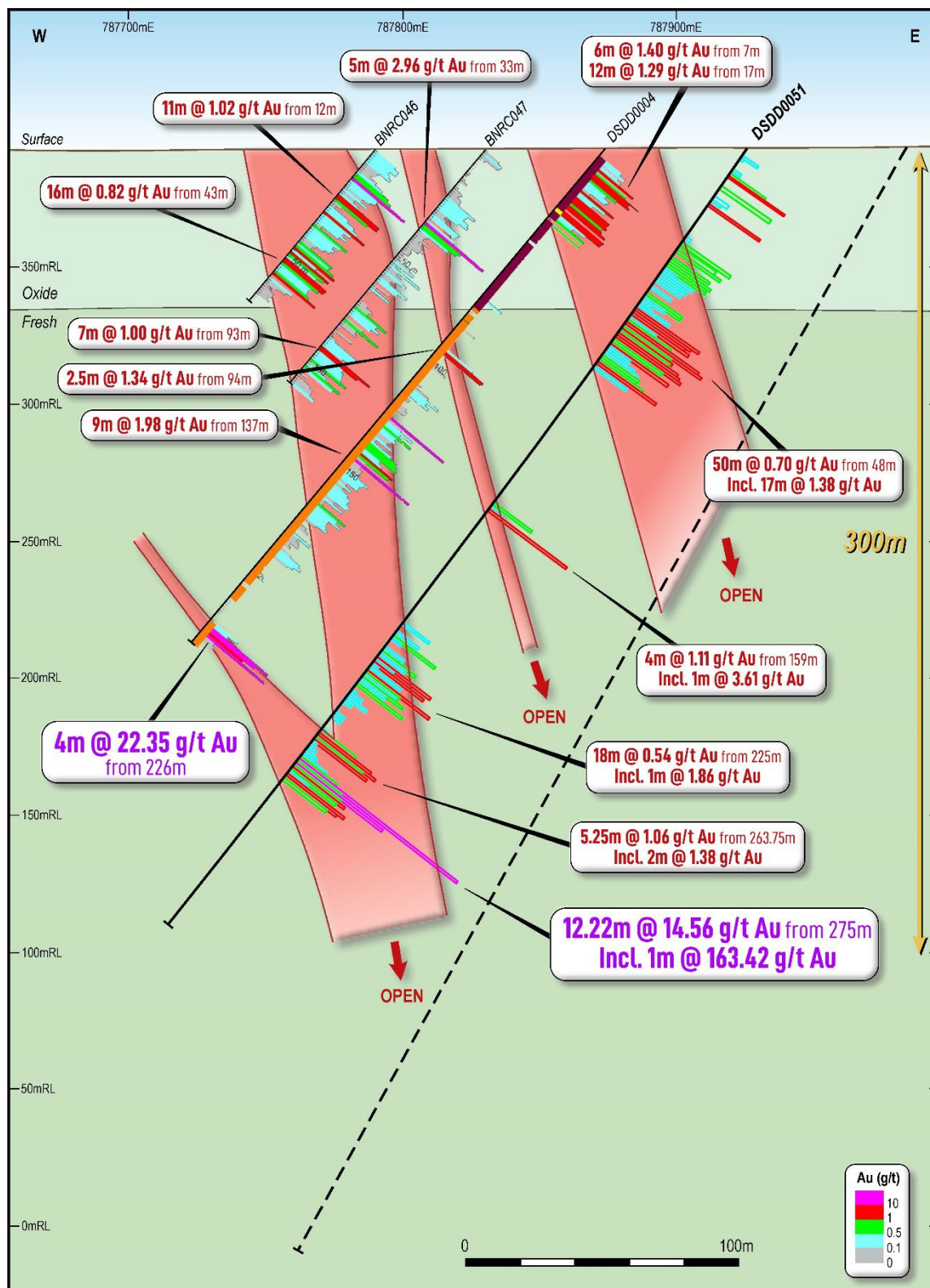
Figure 7: Section 1054500 (+/-25m) showing previous drilling (white) – BD Target 1
