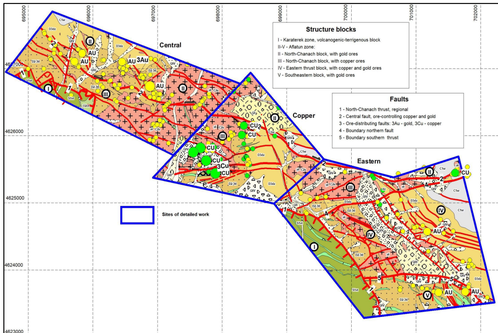
Figure 5: Plan of Tenement - Major Structures from Structural Survey Conducted in 2022
