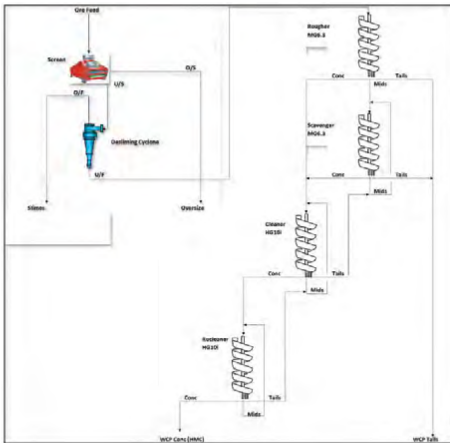
Figure 2.4 Kwale – WCP block flow diagram
