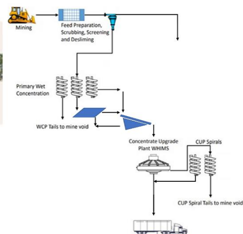
Figure 8: Simple low cost mineral separation plant
