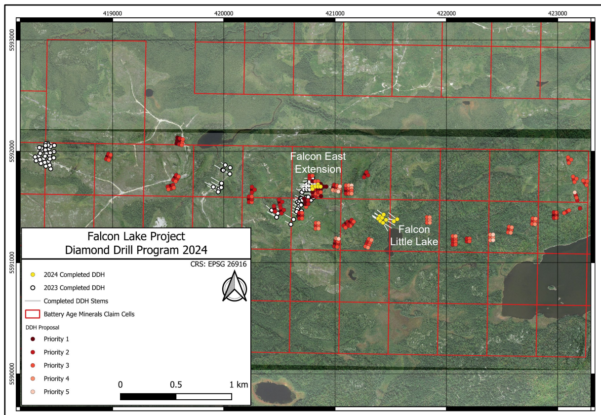
Figure 1 – Plan view of the completed and planned drill hole collars across the Falcon Lake Mineralised corridor
