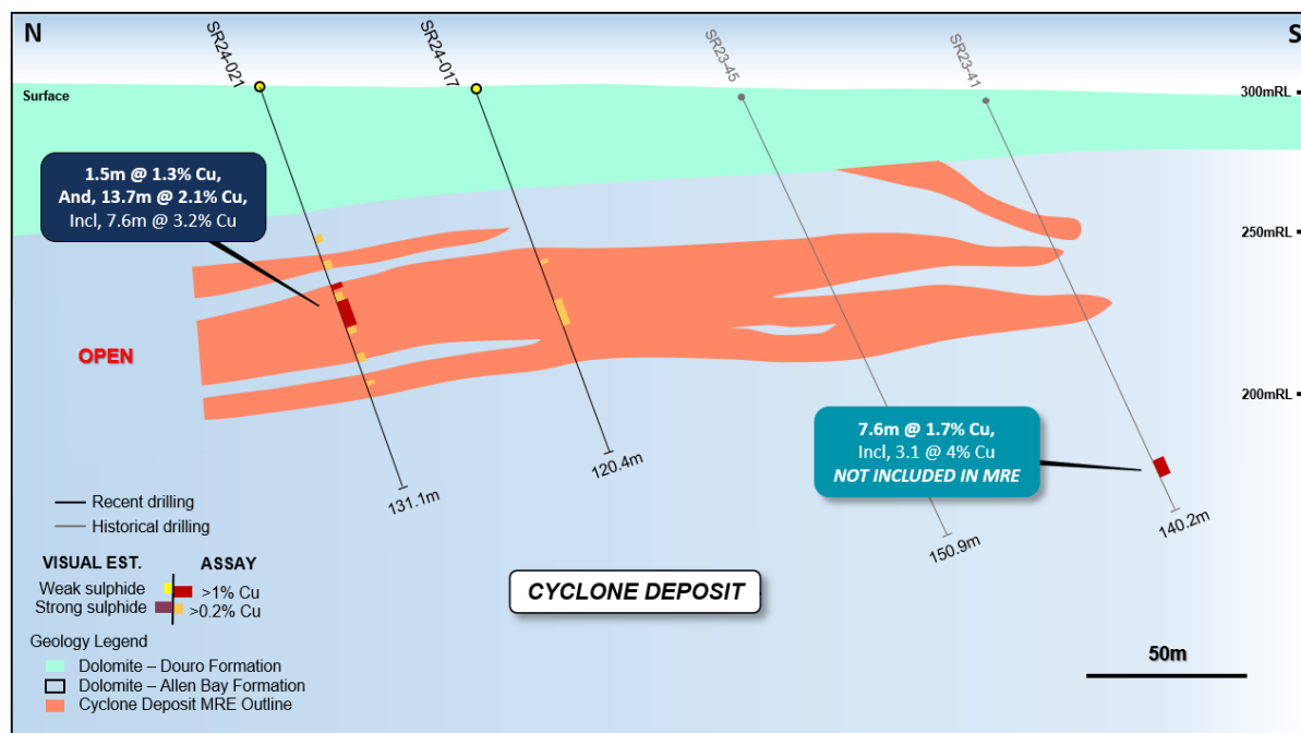
Figure 5: Geological section view at 464,760E showing the mineralised intervals (>0.2% Cu) for drill holes SR24-017 and SR24-021, and the existing Cyclone Deposit resource outline.
