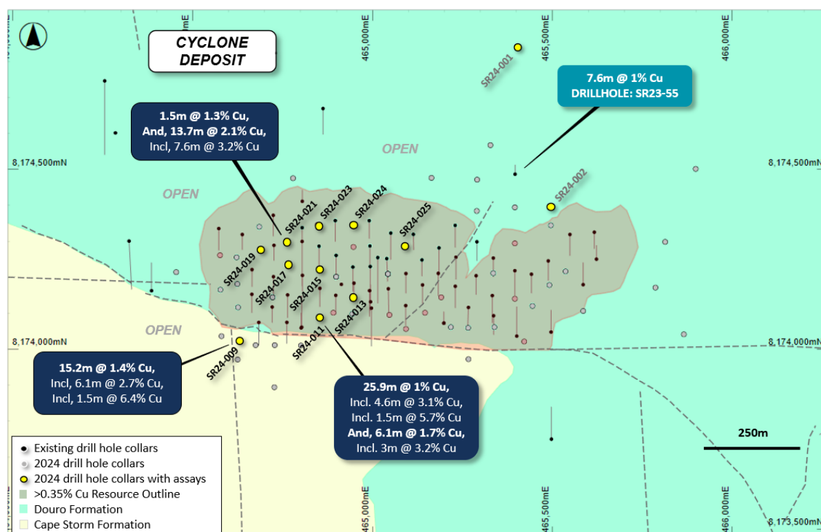
Figure 3: Plan view of the Cyclone Deposit showing the >0.35% Cu resource outline, historical and recent drilling, overlaying regional geology.
