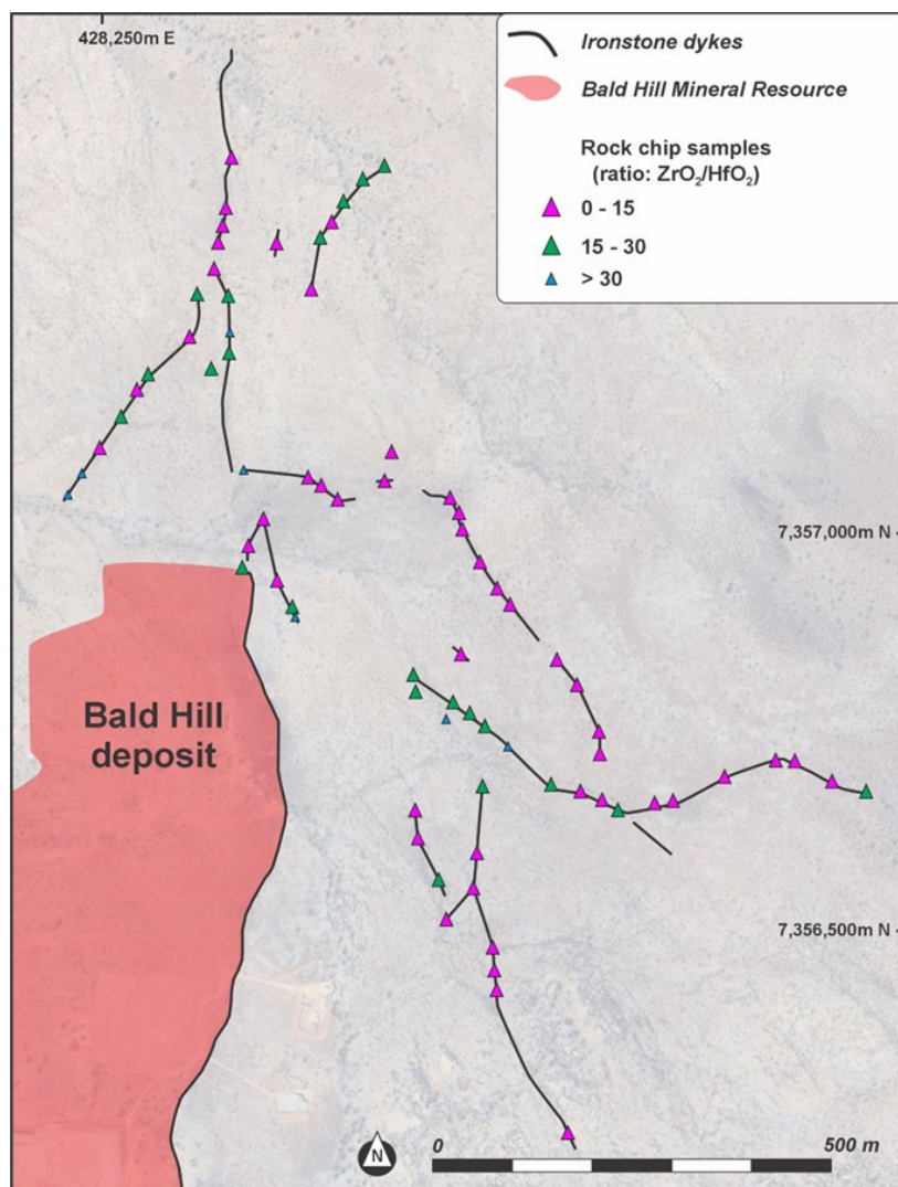
Figure 5: The distribution of ZrO 2 /HfO 2 ratio values for rock chip samples taken of exposed ironstone intrusions to the east and north of the current Bald Hill deposit. Reference is made to Figure 1 for the insert locality. The USGS National Minerals Information Centre states "Zircon is the primary source of all hafnium. Zirconium and hafnium are contained in zircon at a ratio of about 50 to 1." Standard-less semi-quantitative analysis on zircon recovered from Bald Hill samples that were used in process development test work report zirconium and hafnium are contained at a ratio of 13 to 1 (49.05% / 3.78%).
