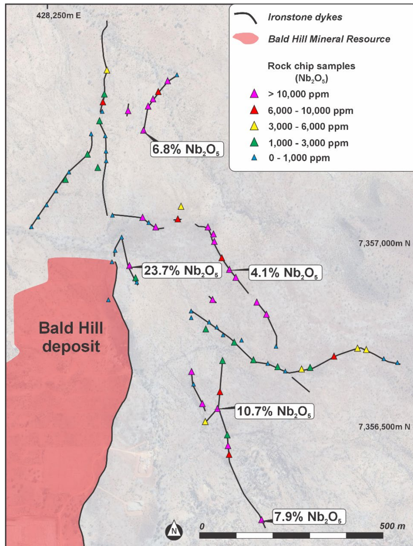
Figure 4: The distribution of \text{Nb}_2\text{O}_5 (%) for rock chip samples taken of exposed ironstone intrusions to the east and north of the current Bald Hill deposit. Reference is made to Figure 1 for the insert locality.
