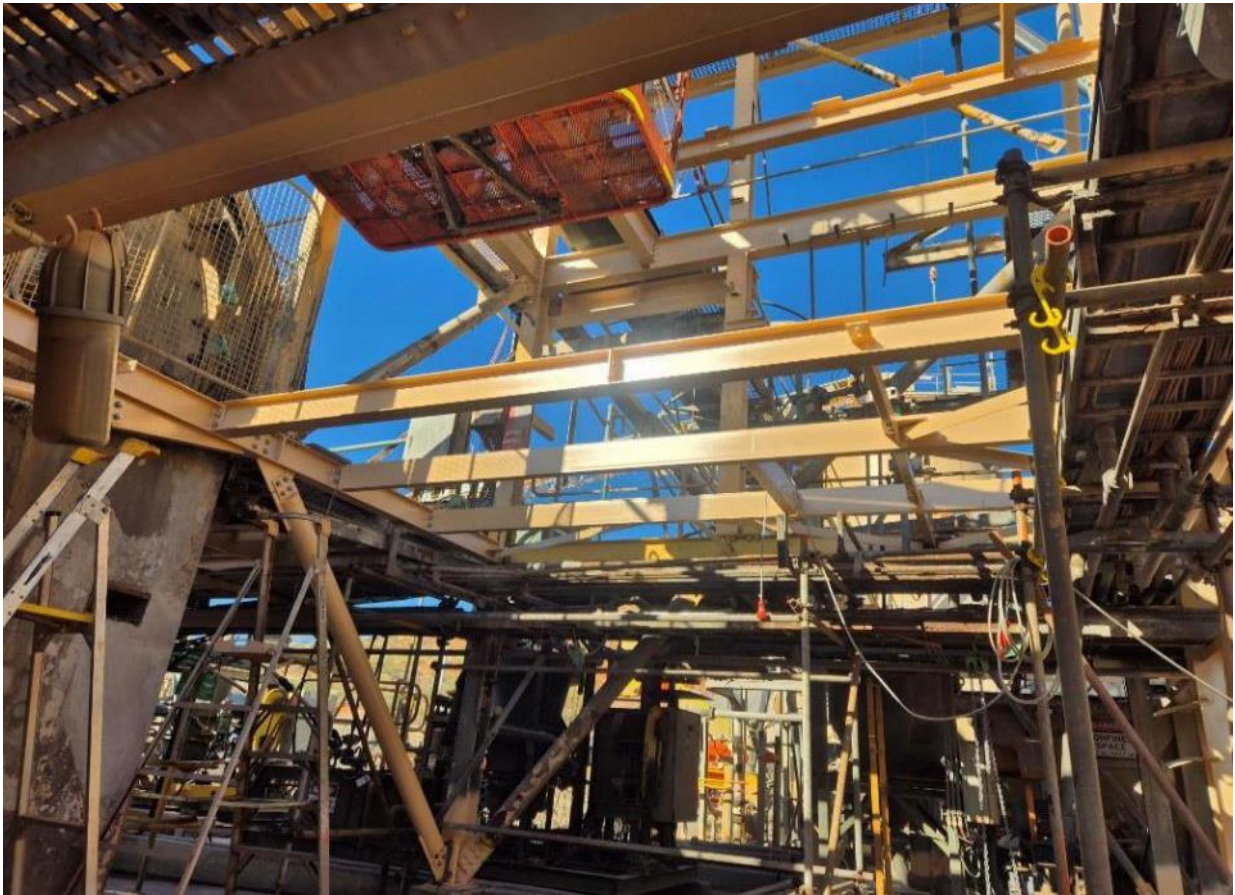
Figure 9: Gravity tower sandblasting completed and steel work installation commenced.
