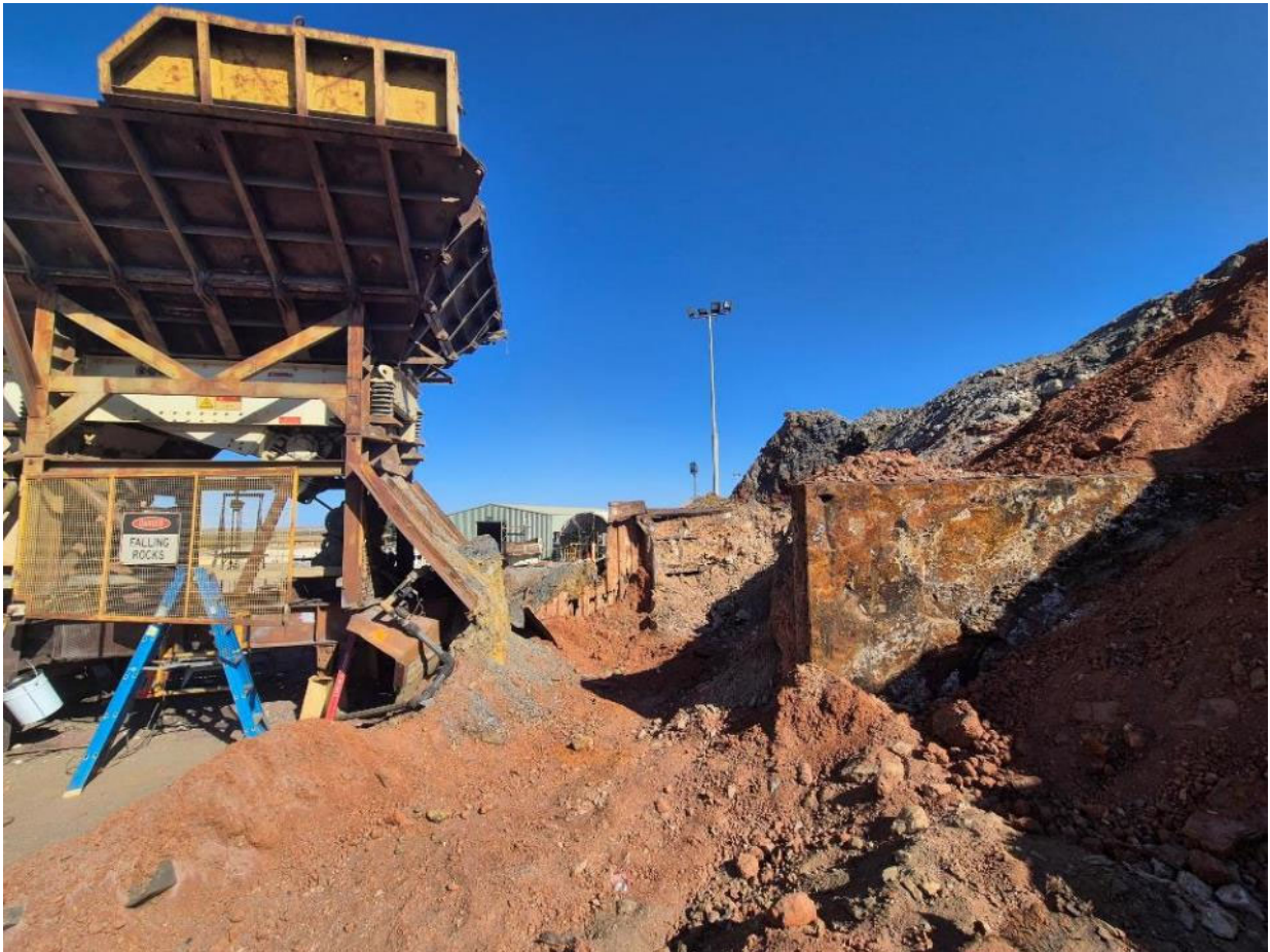
Figure 3: Earthworks completed ahead of installation of the new ROM wall.
