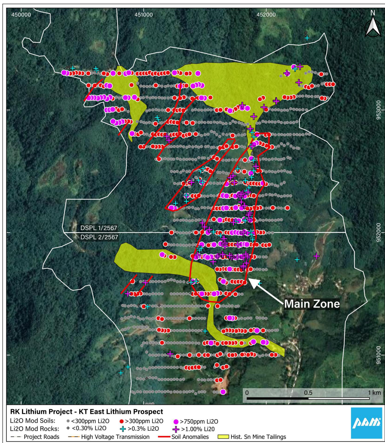
Figure 1: KT East Li Prospect – Soil sampling results
