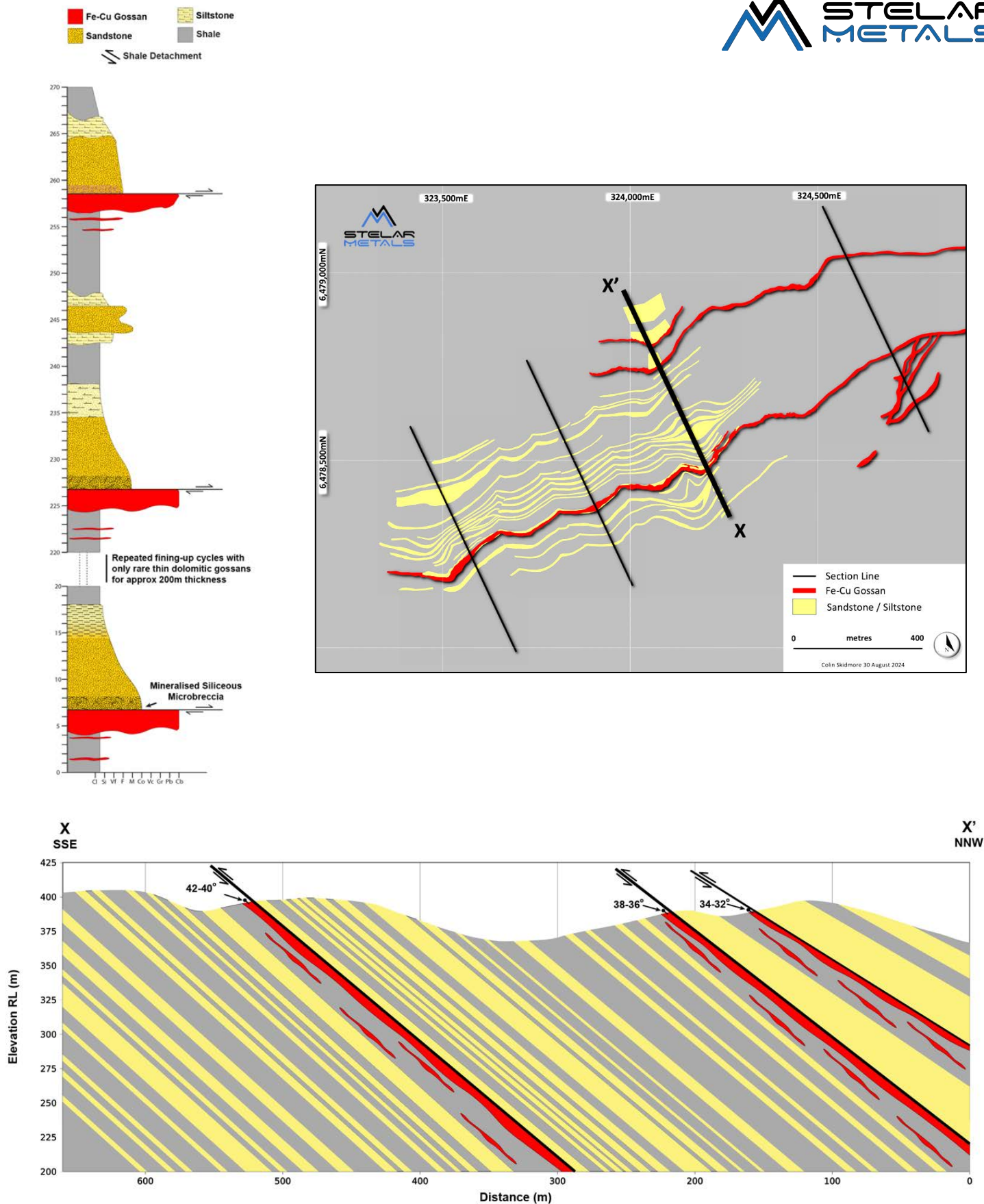
Figure 2: Example measured Stratigraphic Column and Conceptual Cross-section through Baratta Copper Project. (Note: scale varies between Stratigraphic column and cross-section)
