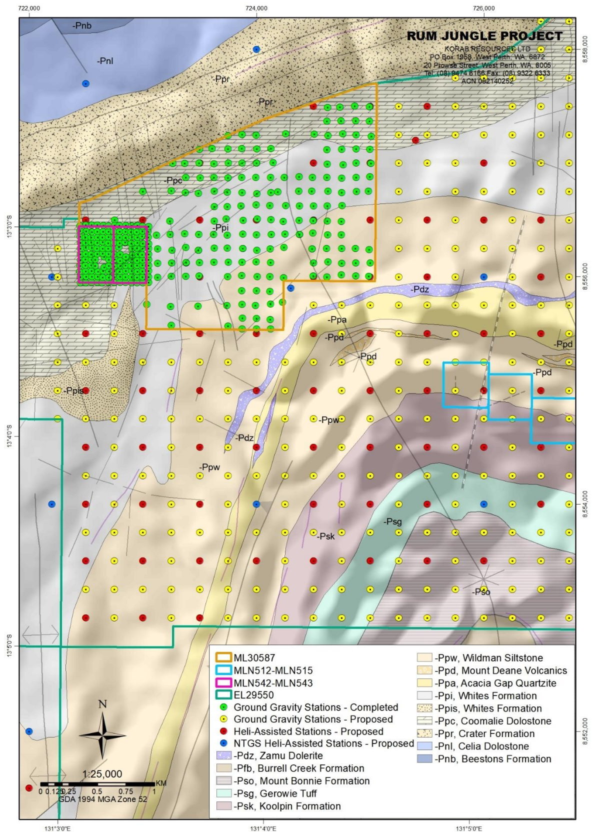
Figure 2 Ground Gravity Survey at Rum Jungle Project - Locations of Survey Stations on Geology
