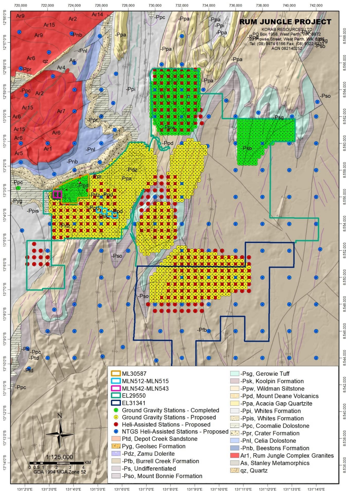
Figure 3 Ground Gravity Survey at Rum Jungle Project - Locations of Survey Stations on Geology
