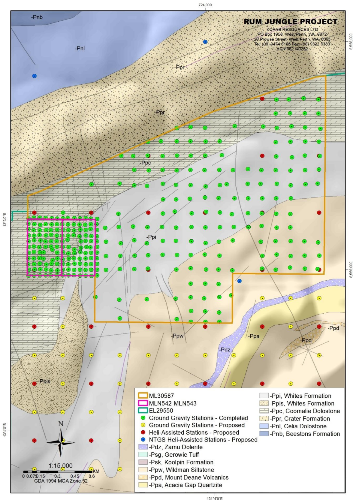
Figure 1 Ground Gravity Survey at Rum Jungle Project - Locations of Survey Stations on Geology
