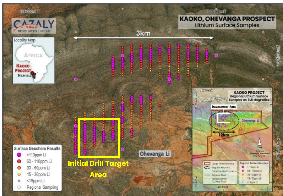
Figure 1. Location of the Ohevanga lithium anomaly and the priority Phase 1 drill target area.
