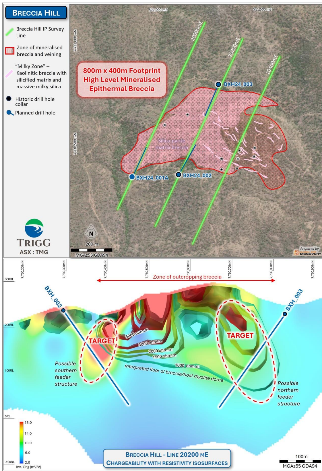
Figure 3: Breccia Hill plan (top) and cross section 20200mE (bottom) displaying 3D IP resistivity inversion iso-surfaces and 2D IP chargeability inversion image, targets and proposed drill holes.
