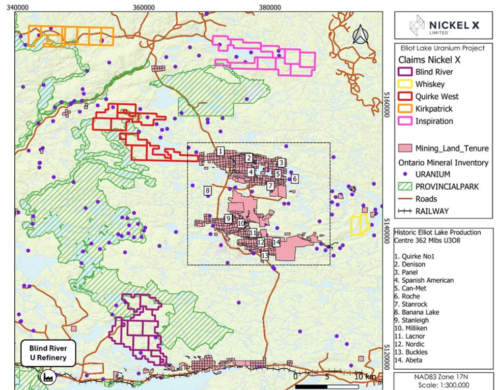
Figure 2. Map of the Elliot Lake Uranium Project and surrounds, also showing the historic Elliot Lake uranium production centre where 362 Mlbs U_3O_8 were mined in the 1950s to 1990s. The Elliot Lake Uranium Project is comprised of five subprojects or claim blocks, known as Blind River, Kirkpatrick, Inspiration, Quirke West and Whiskey.
