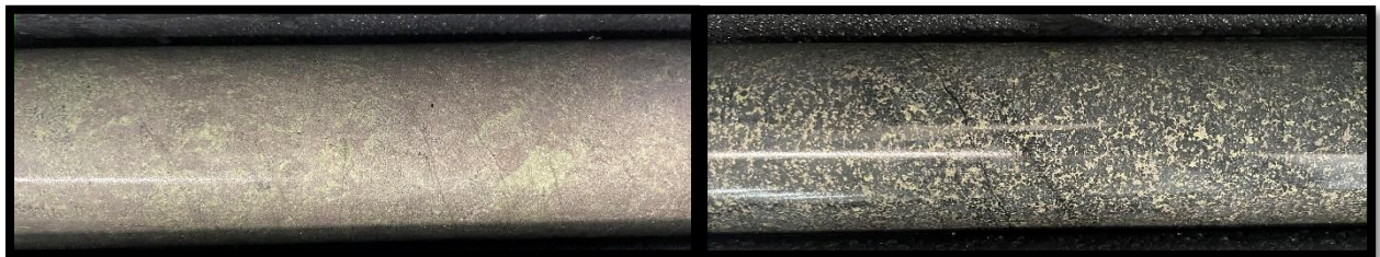
Figure 1. Typical sulphide mineralisation intersected in OVD021: hypogene massive sulphides comprising pyrrhotite-pentlandite-chalcocopyrite at ~110m downhole (left) and matrix/net textured pyrrhotite-pentlandite-chalcocopyrite at ~118m downhole (right).
