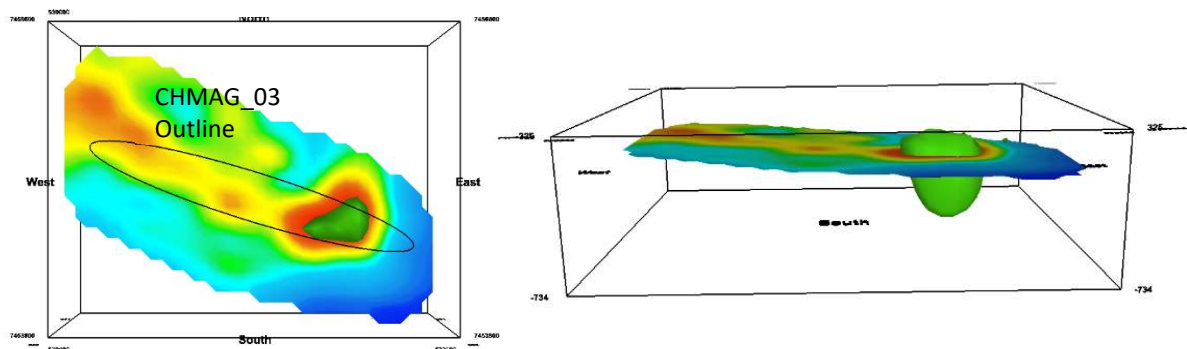
Figure 8. South East gravity survey 3D model result. Looking down through high pass filtered gravity image (left) and looking north (right).
