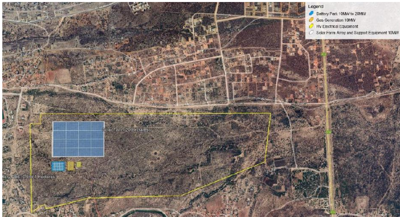
Figure 5 - Schematic of solar and gas hybrid plant layout on Serowe site
