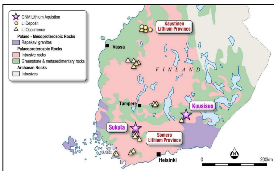
Figure 8: Location of the Sukula project within the Somero Lithium Province and shares similar Paleoproterozoic greenstone and metasedimentary host rocks with the Kaustinen Lithium Province.
