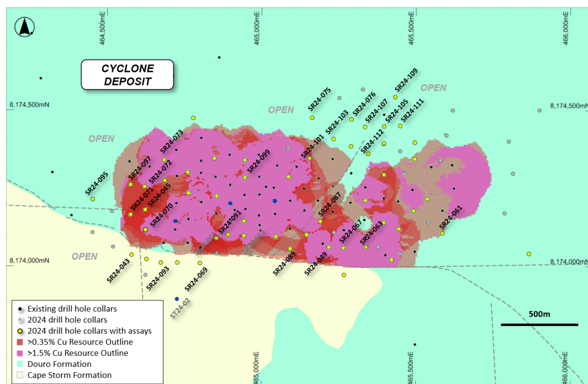
Figure 2: Plan view of the Cyclone Deposit showing the Cu resource outlines, historical and recent drilling, overlaying regional geology.
