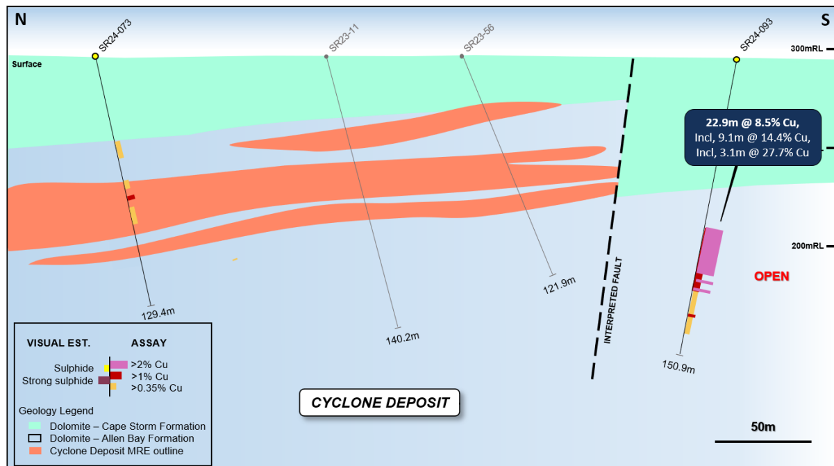
Figure 3: N-S geological schematic section view through SR24-093 and SR24-073 showing the recent drill hole locations, recently received assays, and the current Cyclone Deposit MRE envelope.
