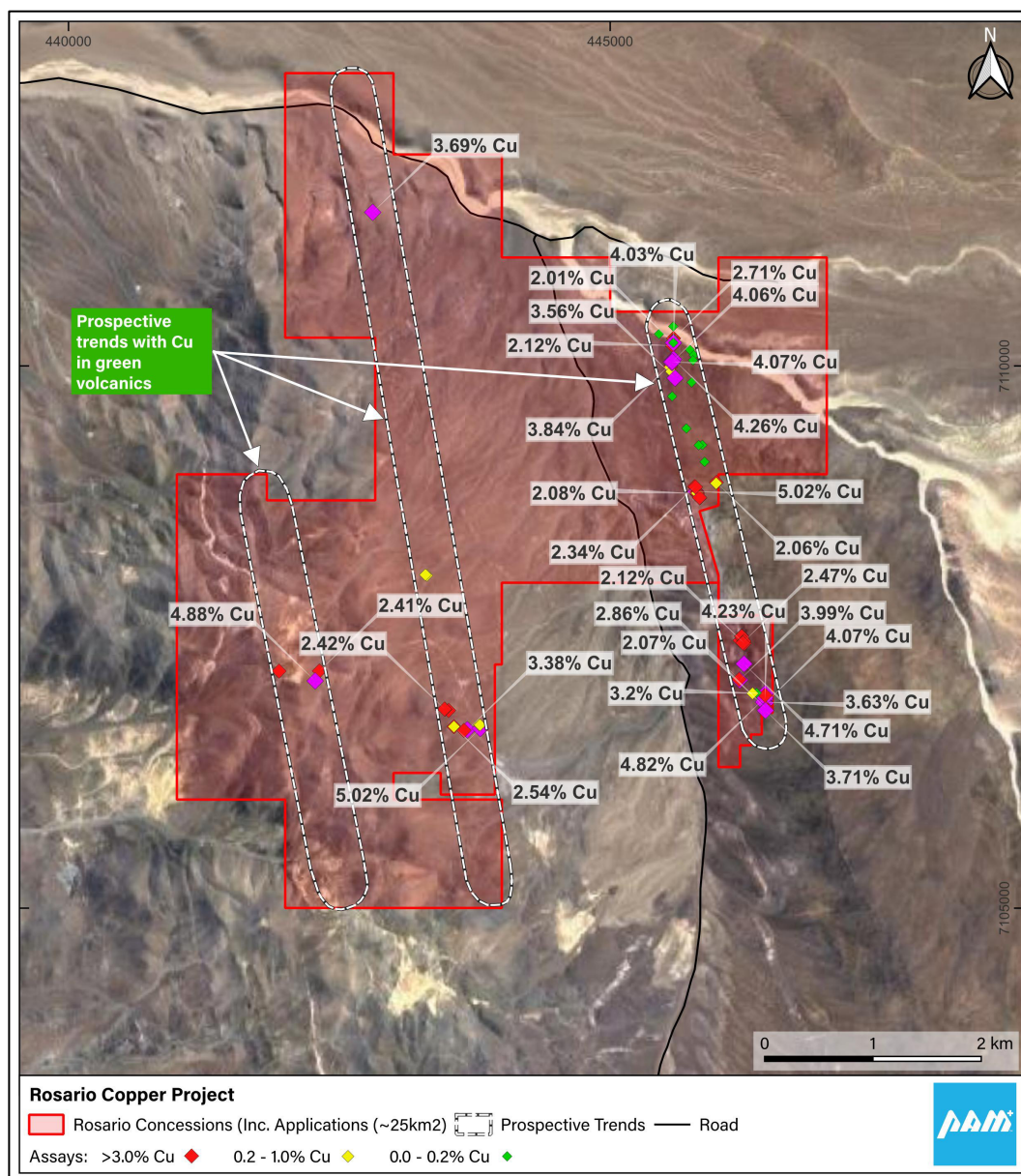
Figure 2: Rosario Copper Project –Geochemistry
