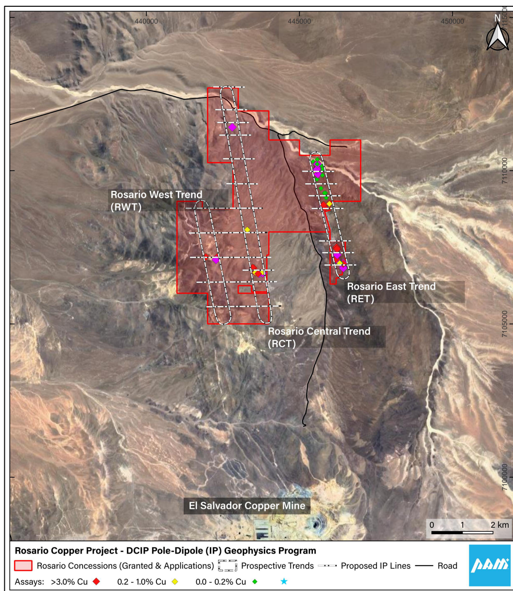
Figure 1: Rosario Copper Project – Proposed IP Survey Lines
