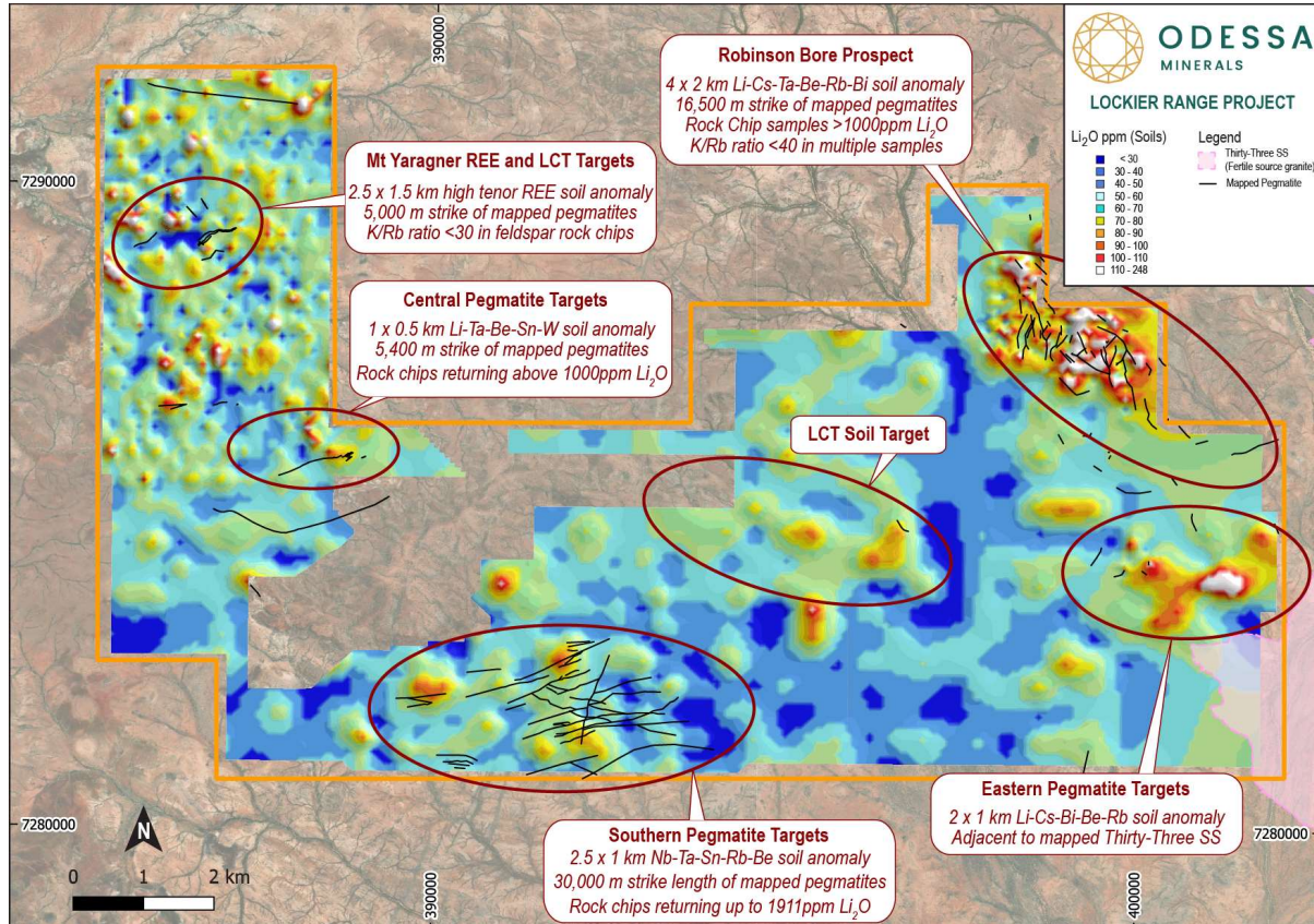
Figure 13: Principal pegmatite target areas within the Lockier Range Project underlain by gridded soil results coded by Li 2 O ppm.
