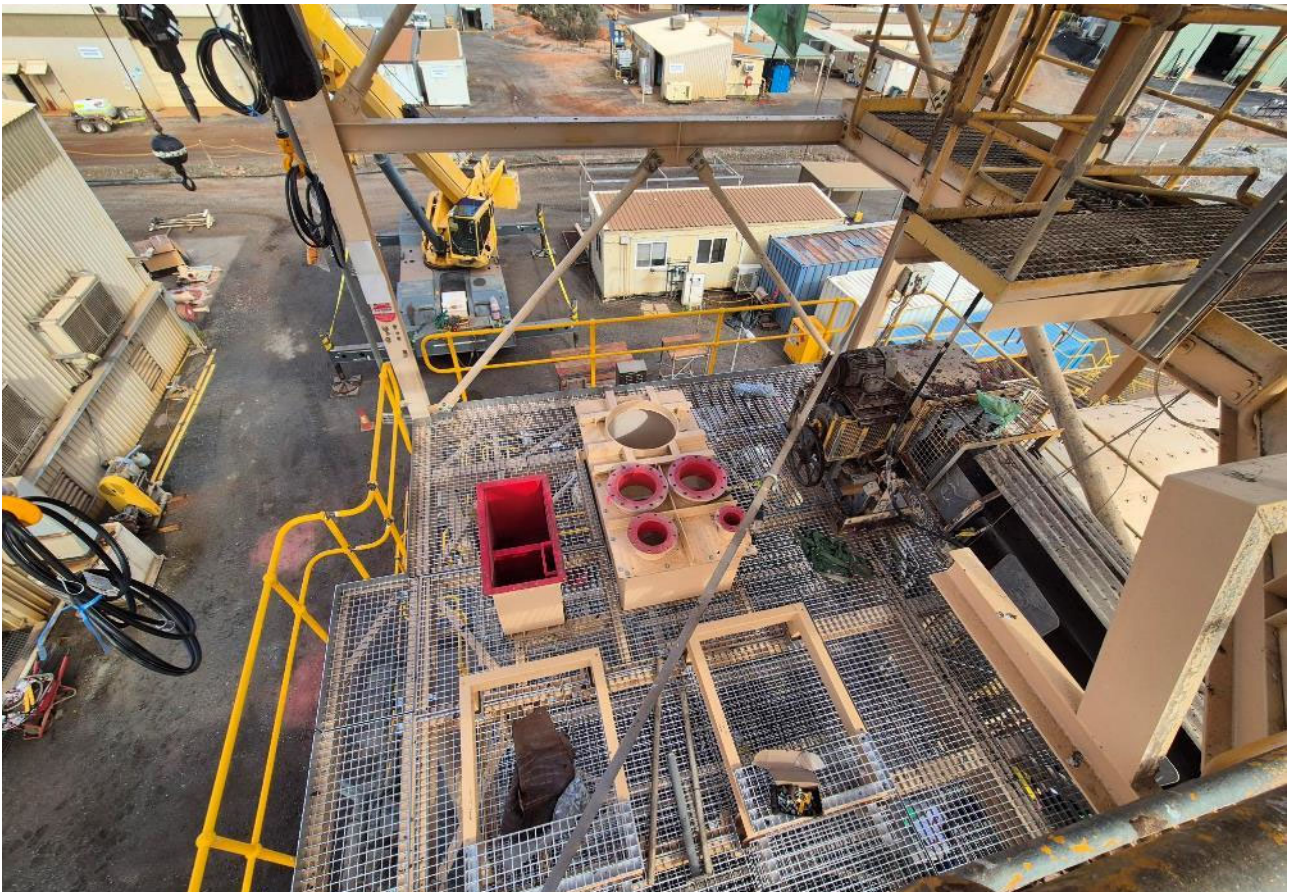
Figure 8: Second deck Knelson stands and boiler box install.
