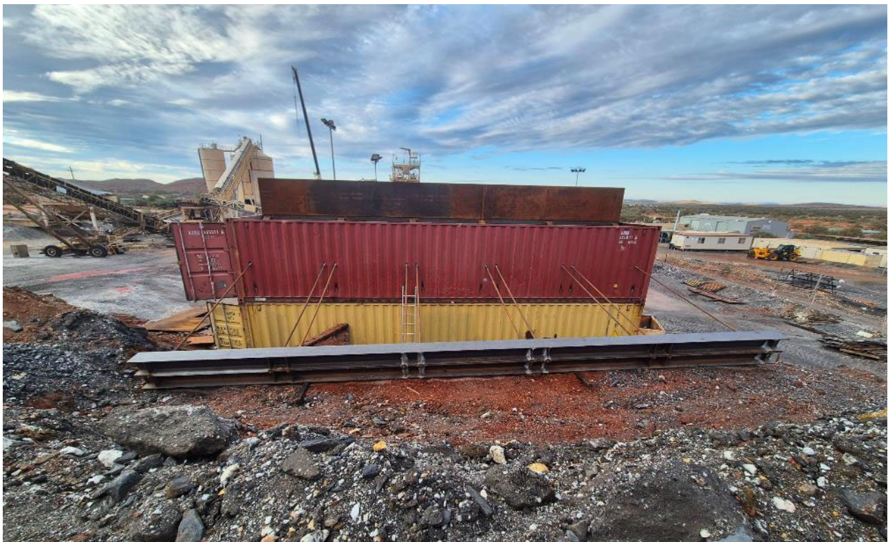
Figure 2: ROM wall installed and awaiting backfill.
