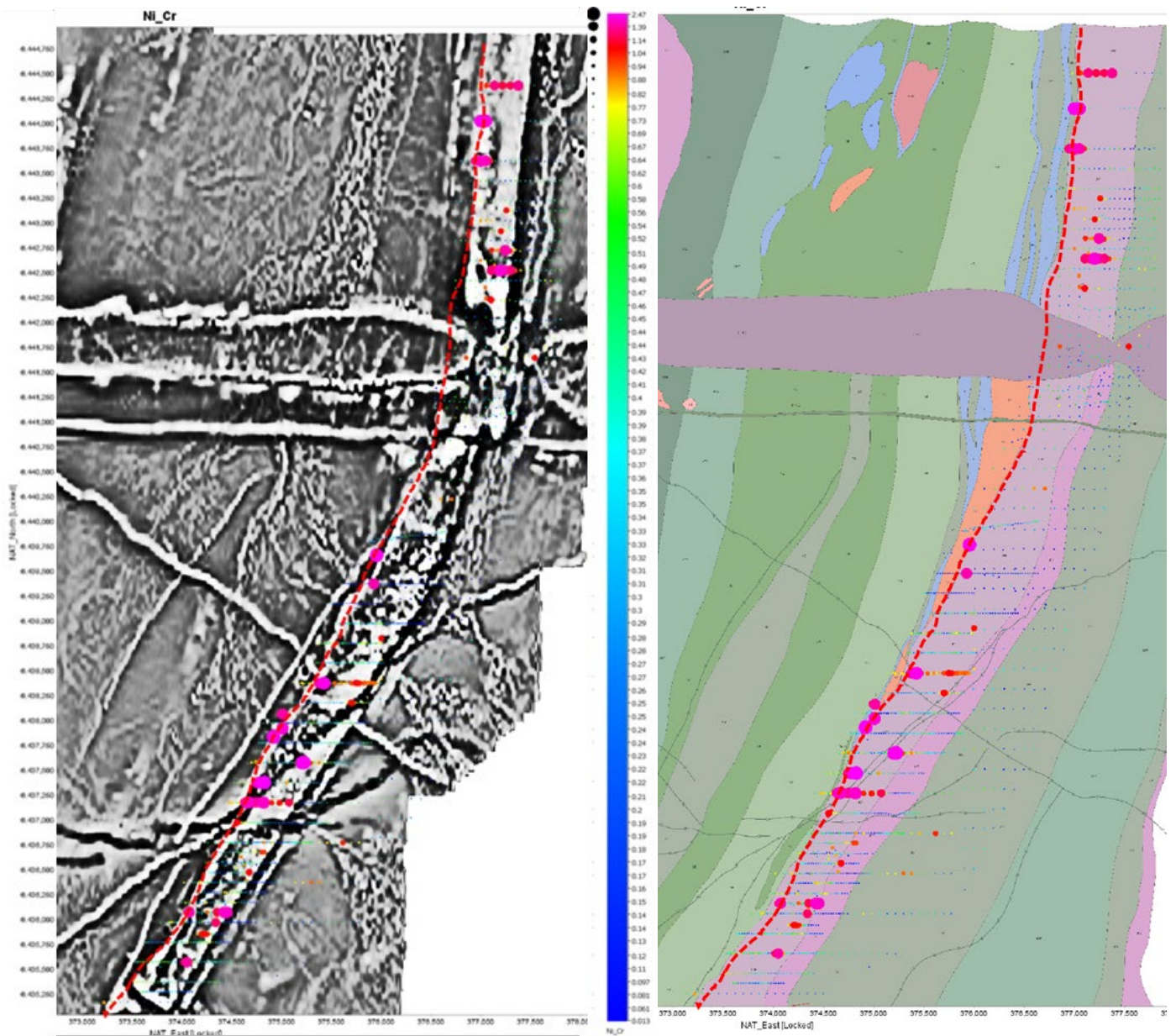
Figure 4 – Ni/Cr ratios at the Mission Sill with magnetic TMI2VD image on the left and 1:10,000 scale mapping on the right. Both Ni/Cr ratios and geological mapping imply the basal unit of the Mission Sill as most prospective for Callisto style sulphide deposits. Red hatched lines on both images shows the position of the basal unit of the intrusive sill complex.
