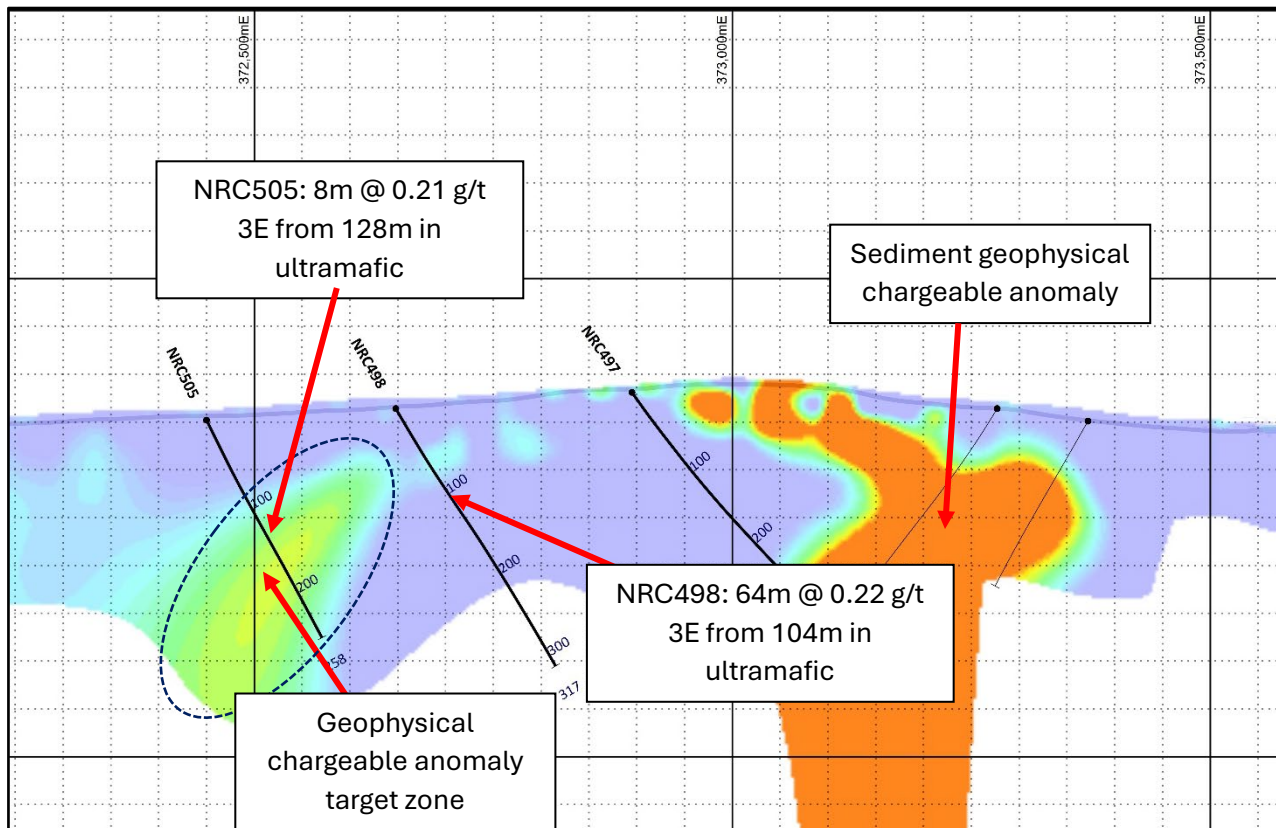
Figure 3 – Chargeability IP model of 6,449,100N (dipole-dipole data) with anomalous drill results in drill hole NRC505 and previous drill hole NRC498.
