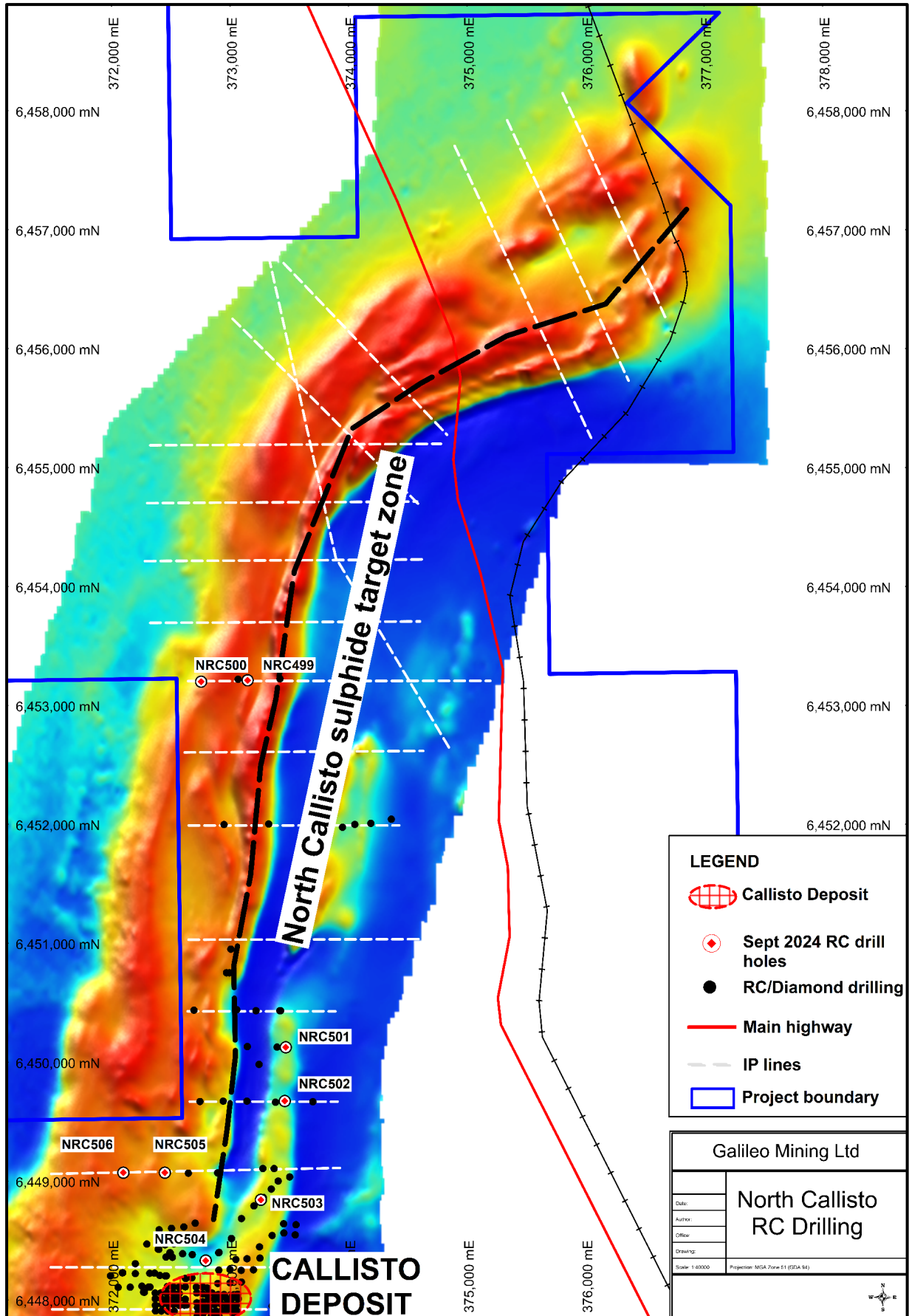
Figure 5 – North Callisto prospect with sulphide target zone and location of recent drilling. TMI magnetic background image.
