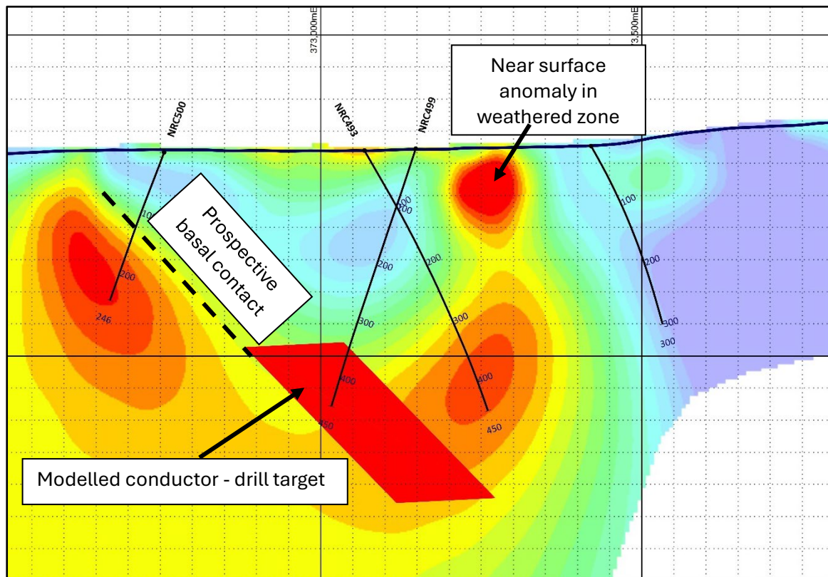
Figure 2 – Modelled conductive target zone and interpreted basal contact unit targeted by NRC499 and NRC500. Resistivity background image (low resistance = red colour, related to higher conductivity zones)
