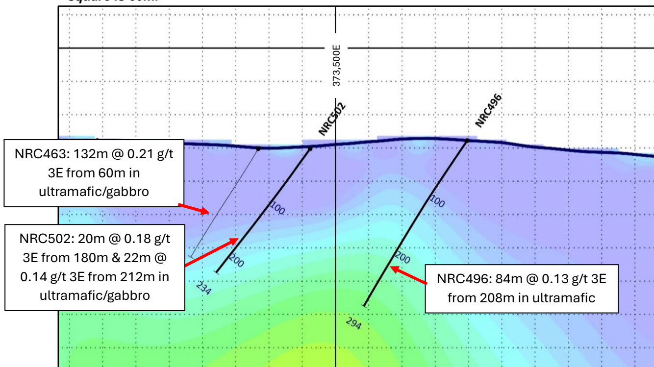
Figure 1 –Chargeability IP model of 6,449,700N with anomalous drill results in NRC502 and previous drill results at the contact between ultramafic and gabbroic rocks units. Each hatched square is 50m.
