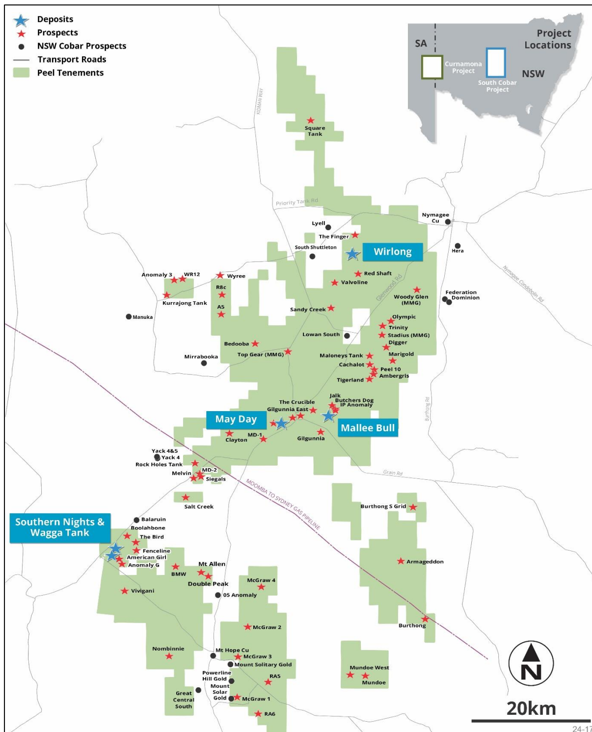
Figure 8 – Peel Cobar Basin tenure and prospects
