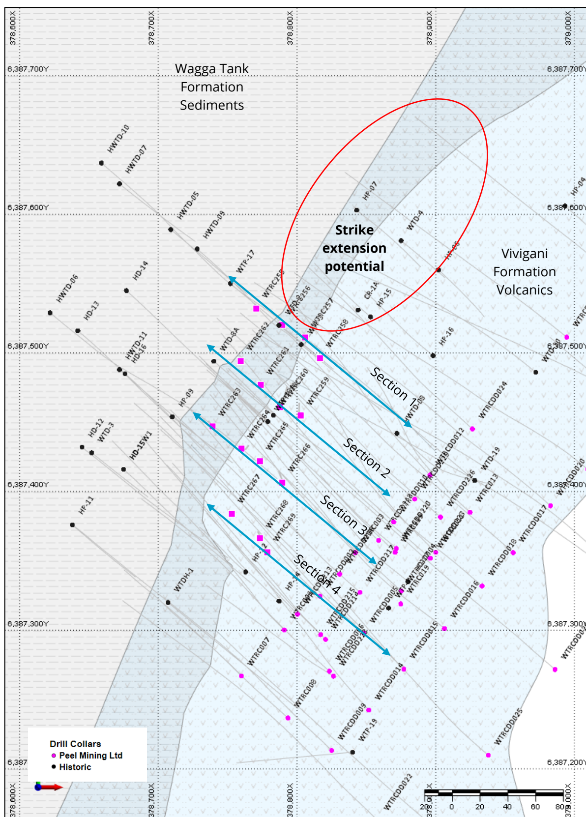
Figure 2 – Wagga Tank Drilling over chargeability ~160m below surface (Magenta = Peel; black = historic)
