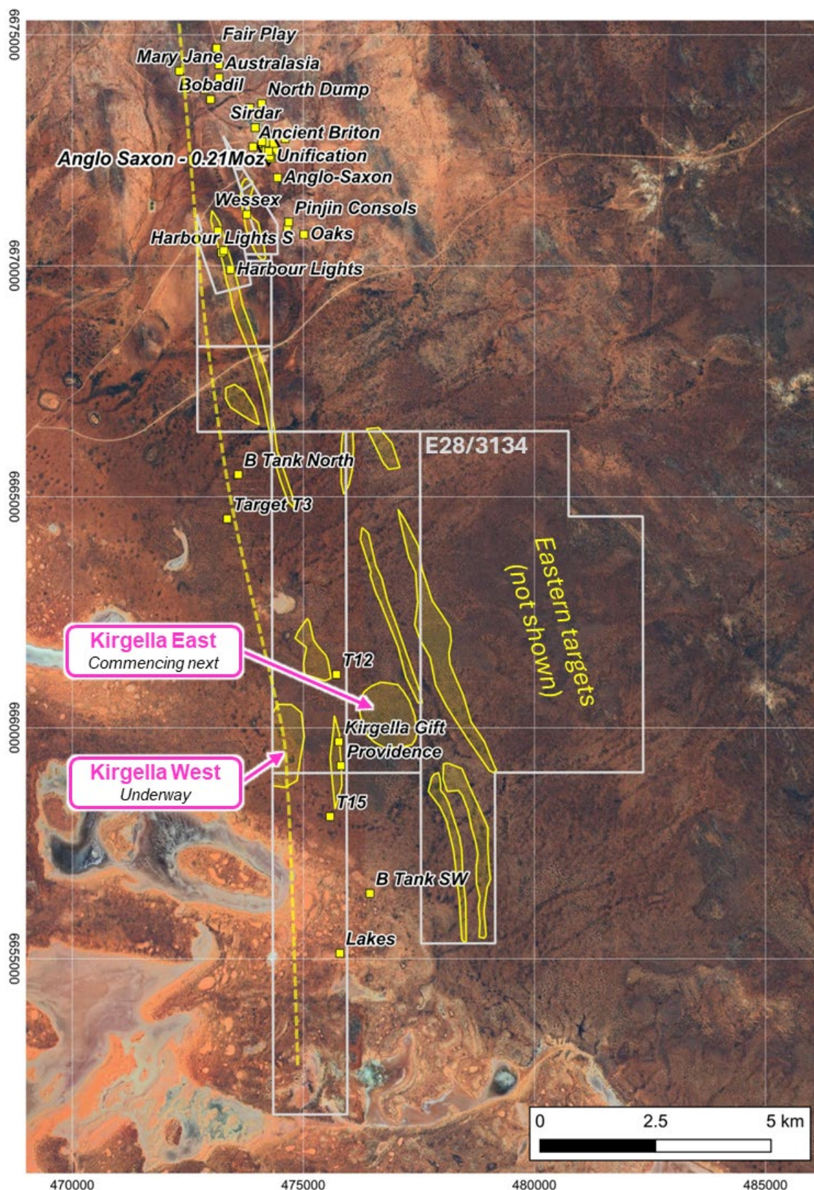
Figure 3 – Some of the exploration target areas (yellow) marked for upcoming exploration programs. Most areas include clusters of targets that are elongate along the trend of the Laverton Tectonic Zone. Eastern targets on E28/3134 (labelled but not shown) are located in potentially high grade metamorphic rocks (?Rebecca equivalents?) in sheared contact with the Pinjin sequence. Drilling is underway at Kirgella West, and will commence shortly at Kirgella East. Projection: MGA 94 Zone 51.
