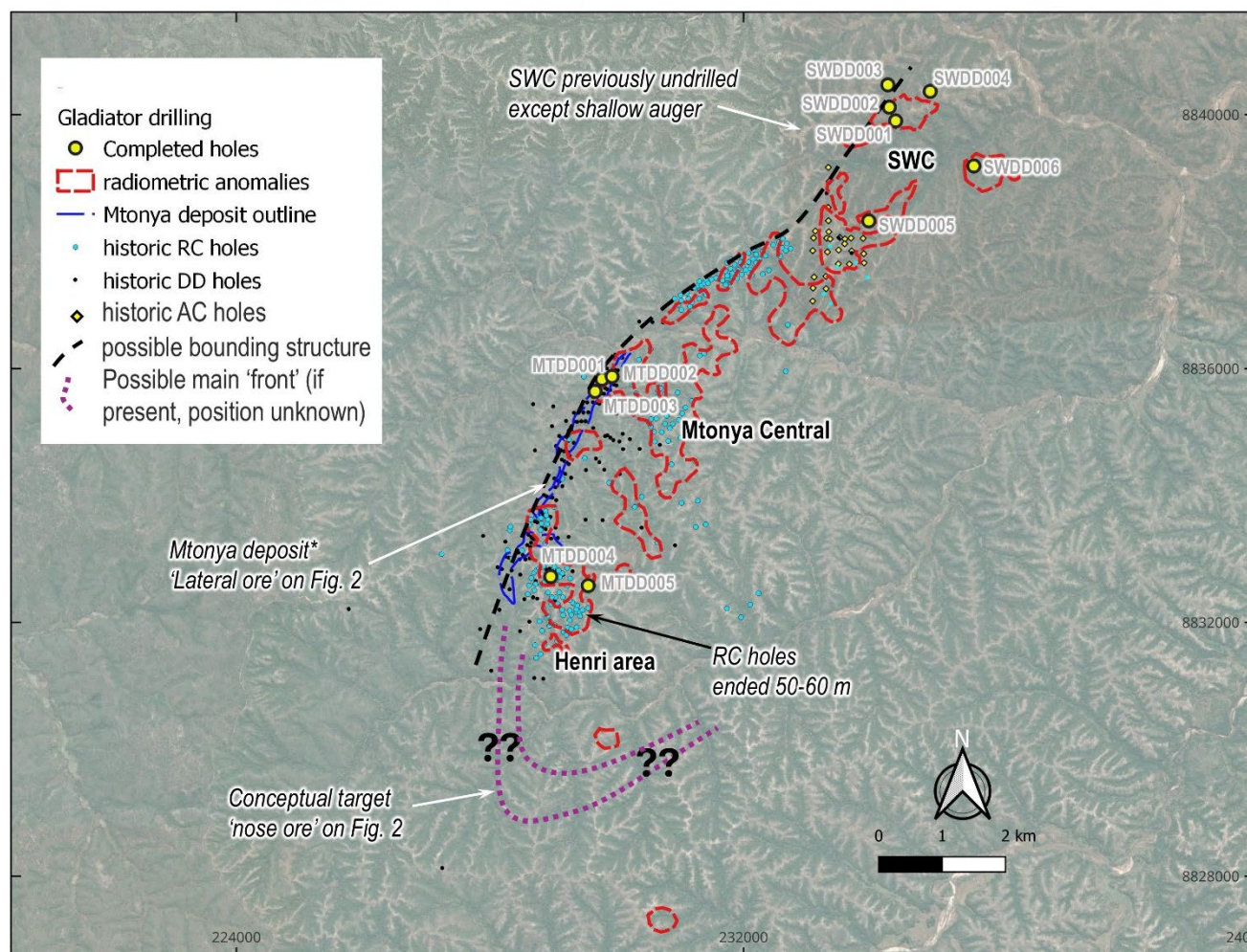
Figure 3: Map of the SWC and Mtonya targets showing historic and Gladiators drilling
