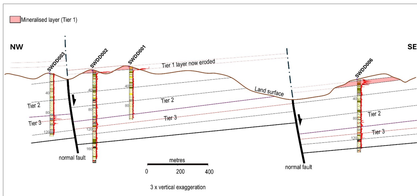
Figure 4: Cross-sectional interpretation through SWC
