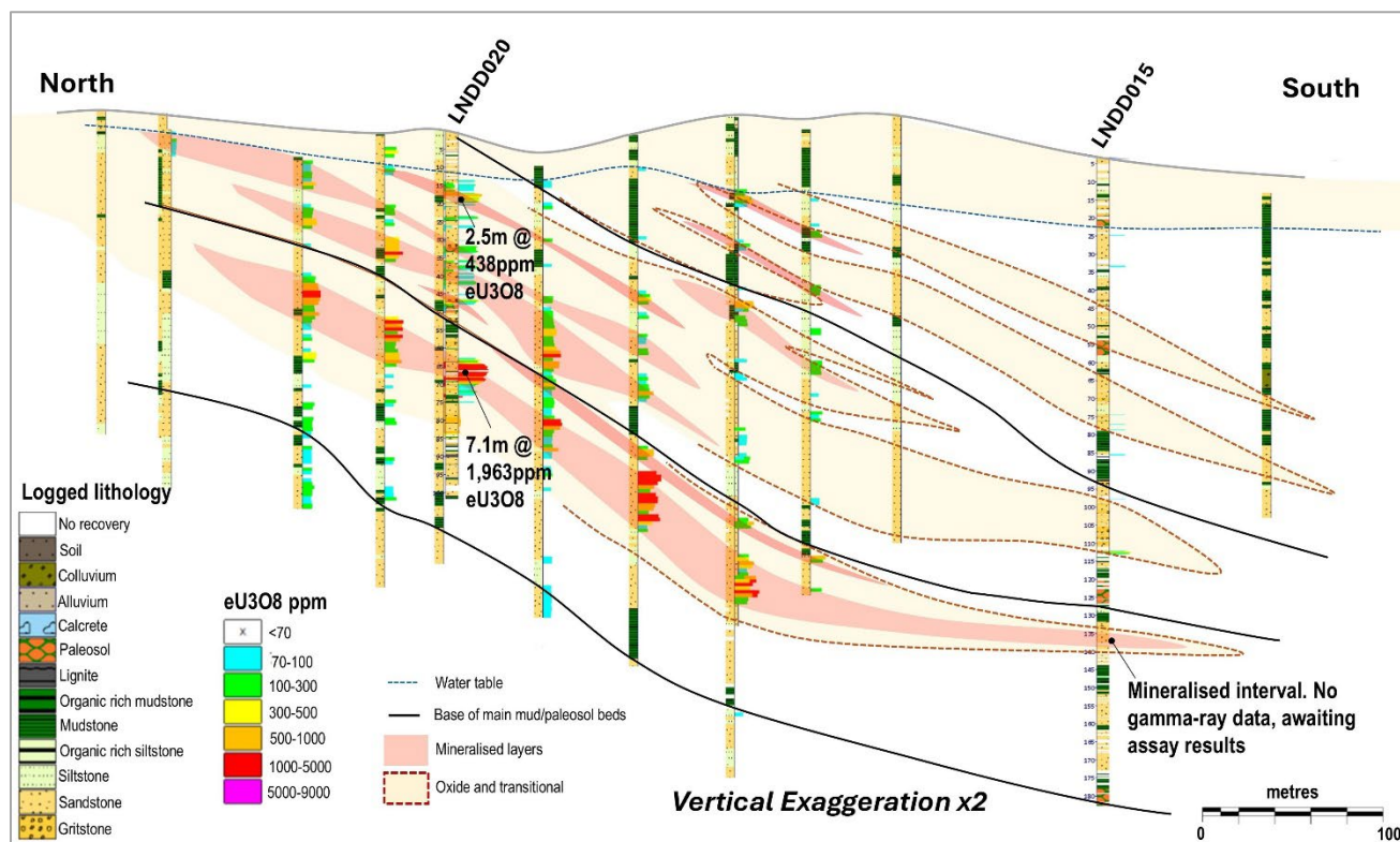
Figure 6: North-south cross-section showing the downhole logged eU3O8, mineralized layers and oxide/transitional zones. LNDD015 and LNDD020 are shown.
