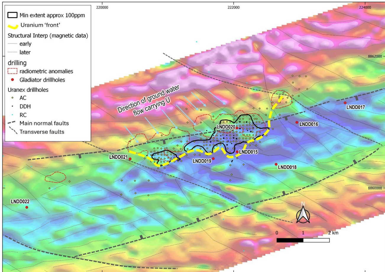
Figure 5: Ground magnetic image (1VD) with the Likuyu North deposit shown along with the interpreted 'uranium-front' and main structures. Gladiators' recent holes are shown.
