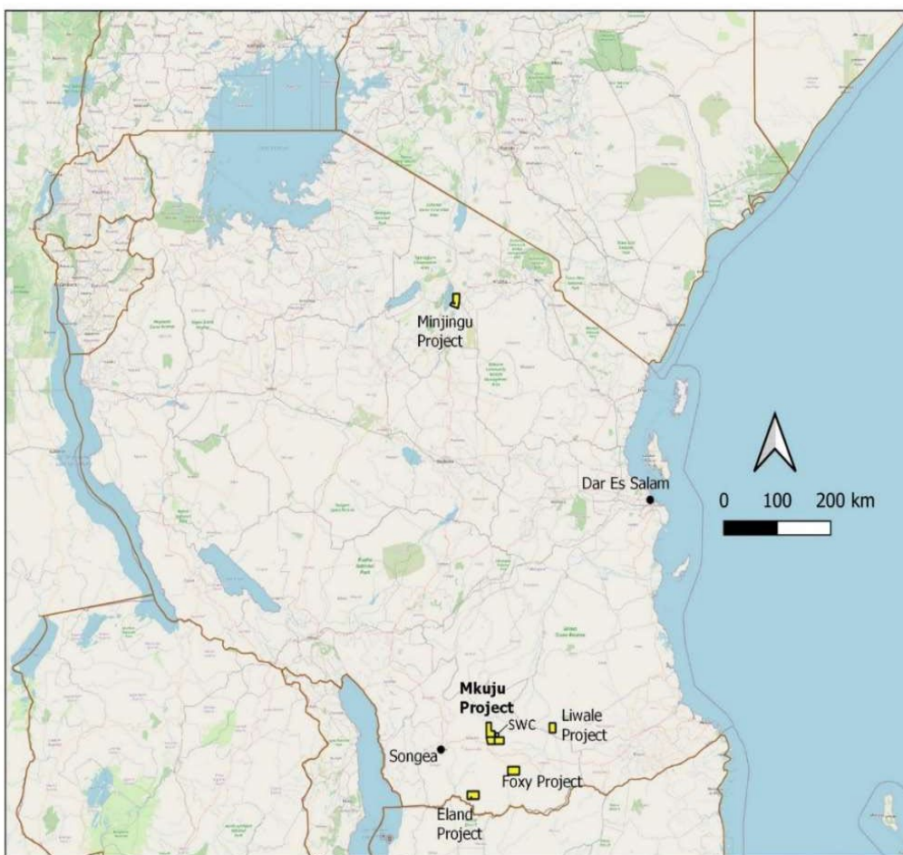
Figure 1: Prospecting Licenses held by Zeus Resources (T) Limited in Tanzania.
