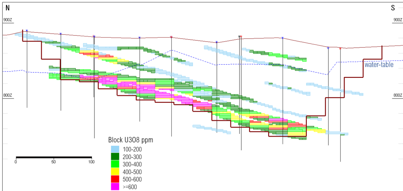
Figure 8: Cross section through the Likuyu North deposit along the line of section drawn on Figure 7 .
