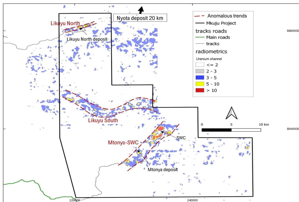
Figure 2: The Mkuju Project area over airborne radiometric data with important deposits and targets labelled. The new SWC license is also shown.
