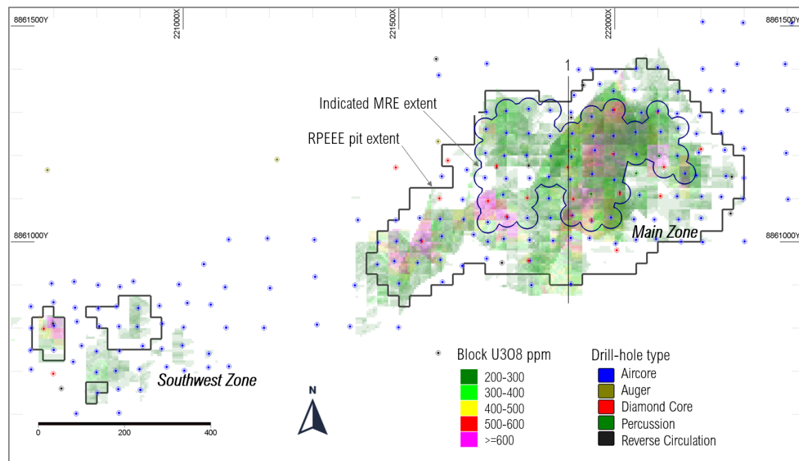
Figure 7: Plan view of the block model for Likuyu North and line of cross section in Figure 8.
