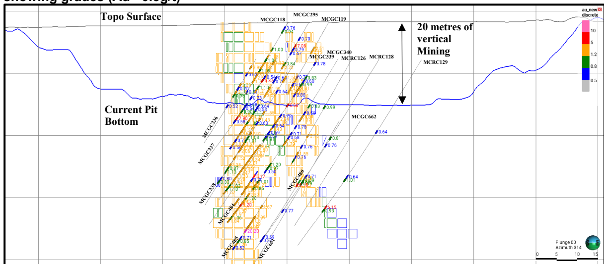
Figure 18: Cross section 2 looking Northwest – Kangaroo Bore Pit block model and drillhole assays showing grades (Au >0.5g/t)
