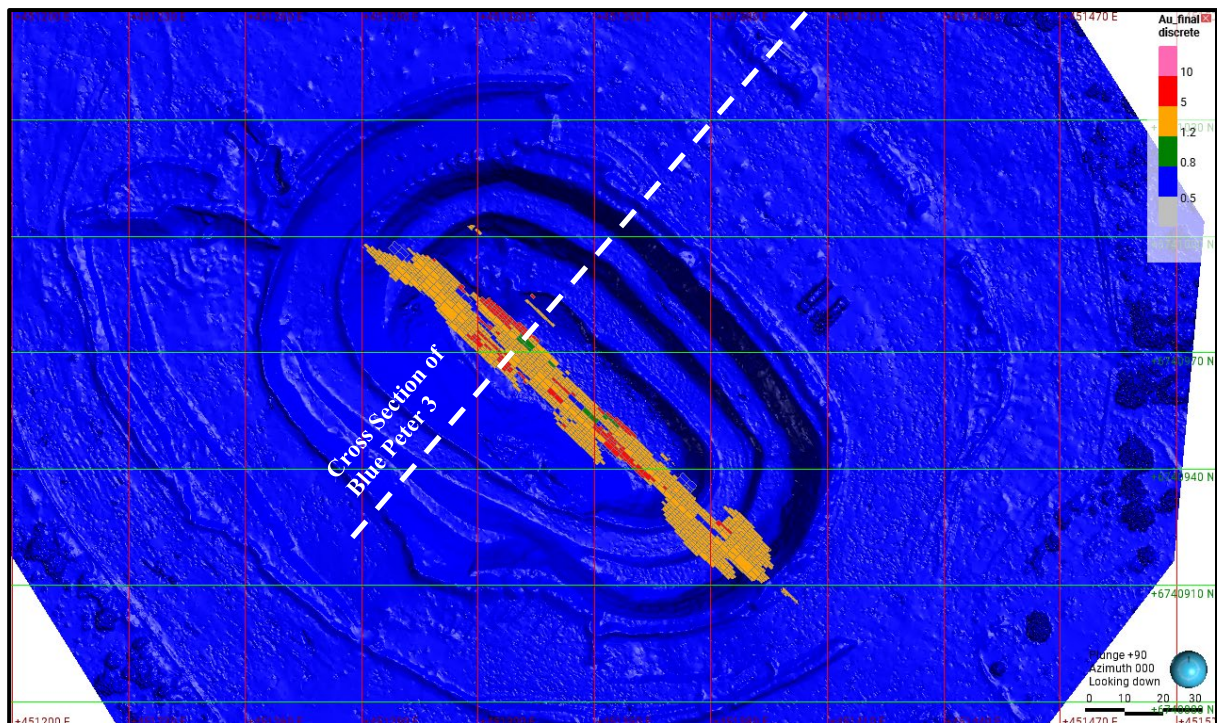
Figure 14: Plan section– Blue Peter 3 Pit showing section lines and block model
