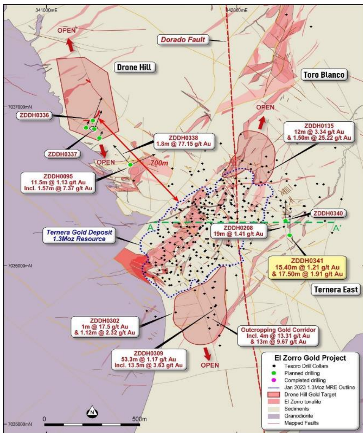
Figure 2: Ternera area drill locations in current program, location of hole ZDDH0341 within the Ternera East target, and significant results showing areas of open gold mineralisation close to Ternera (refer ASX Announcements 2 July 2024, 23 March 2021, 25 June 2021, 3 November 2021, 8 November 2022, 18 September 2023, and 13 June 2024). Section location for Figure 2 shown at A-A' - Datum PSAD56 19S.
