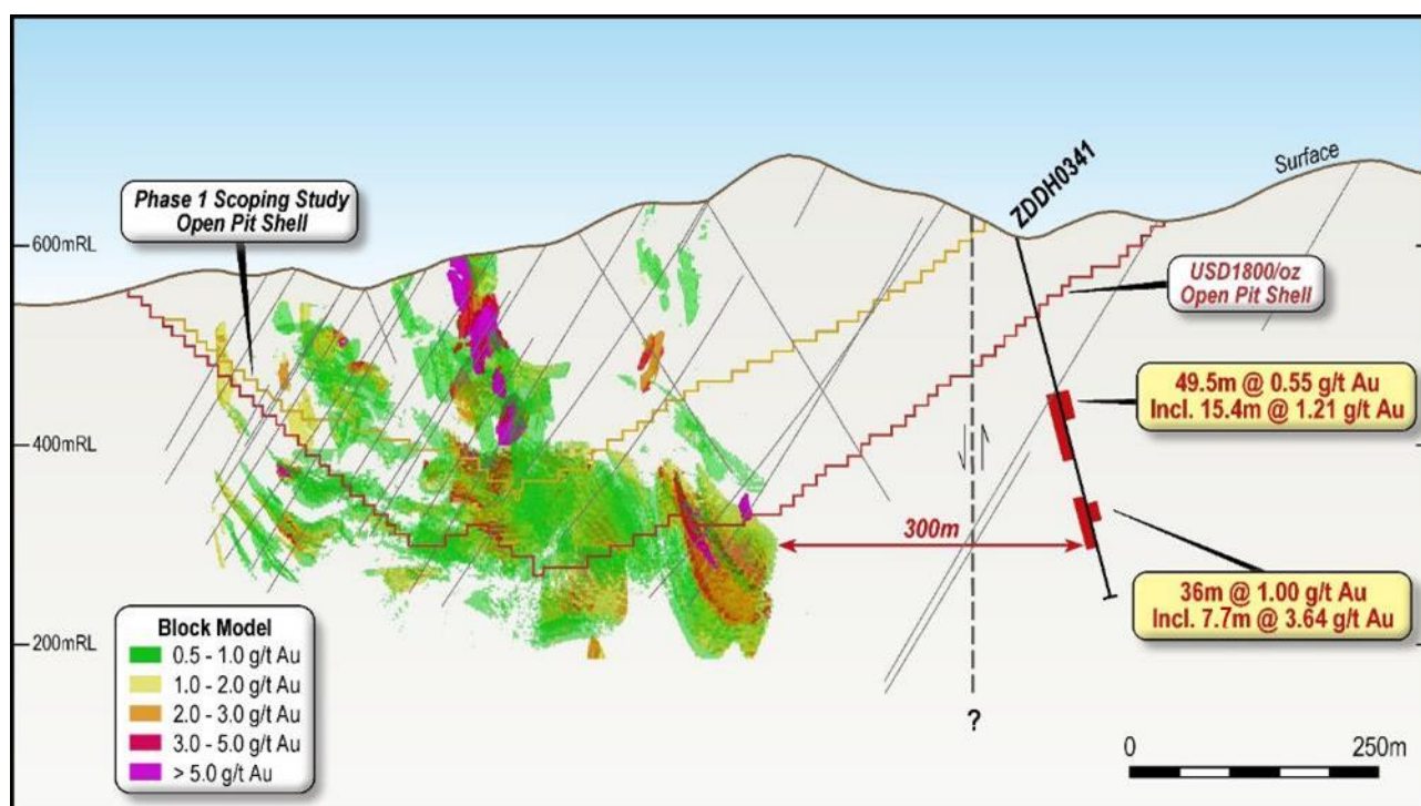
Figure 3: Ternea East drilling, ZDDH0341 showing significant mineralised zones and location relative to the Ternea Gold Deposit MRE Block Model and USD1800 optimised Pit Shell., looking north. Hole ZDDH0341 was drilled toward 000 and is projected onto section. Previous drilling shown as pale grey drill traces. Refer ASX announcement 6 December 2021 for hole ZDDH0223 results, and ASX Announcement 2 July 2024.
