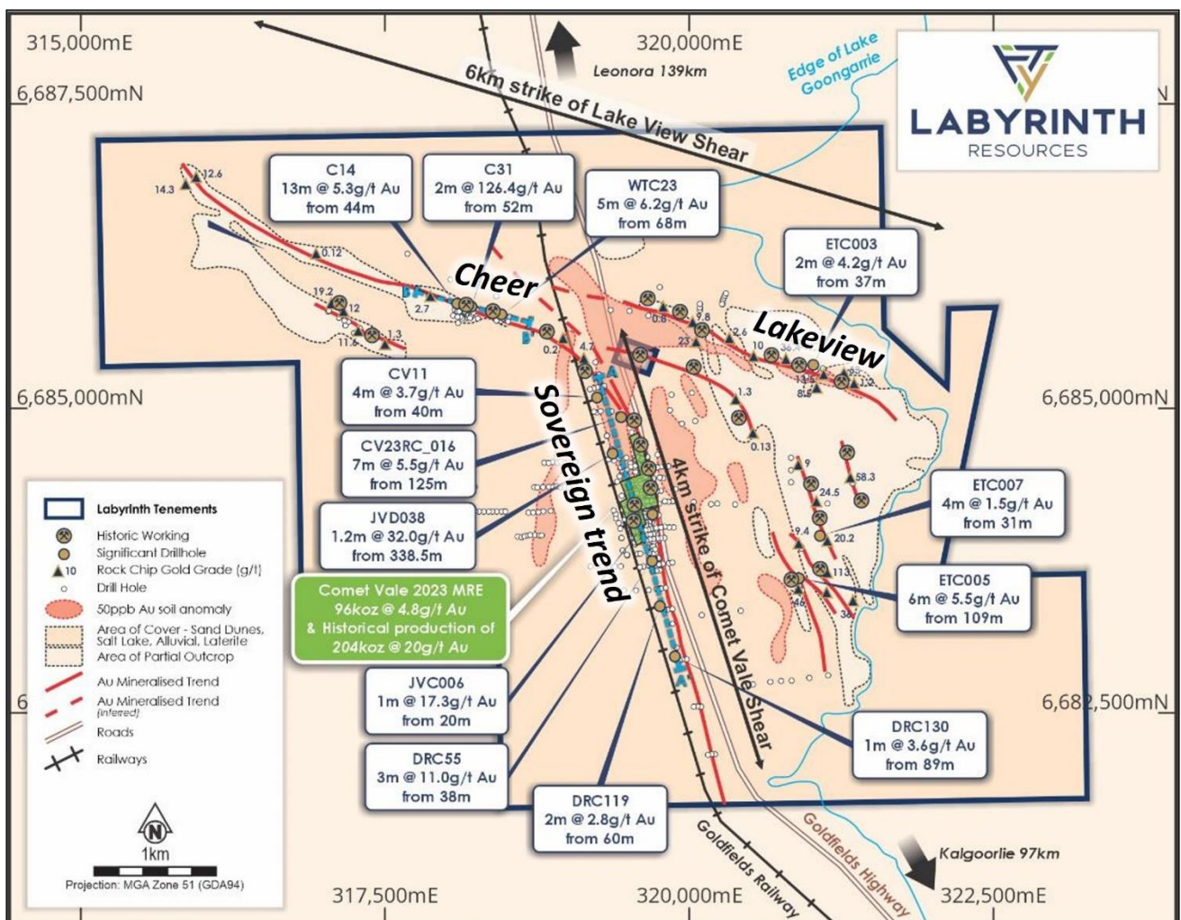
Figure 1. Plan View of Comet Vale Project drilling targets and significant historic intercepts.
