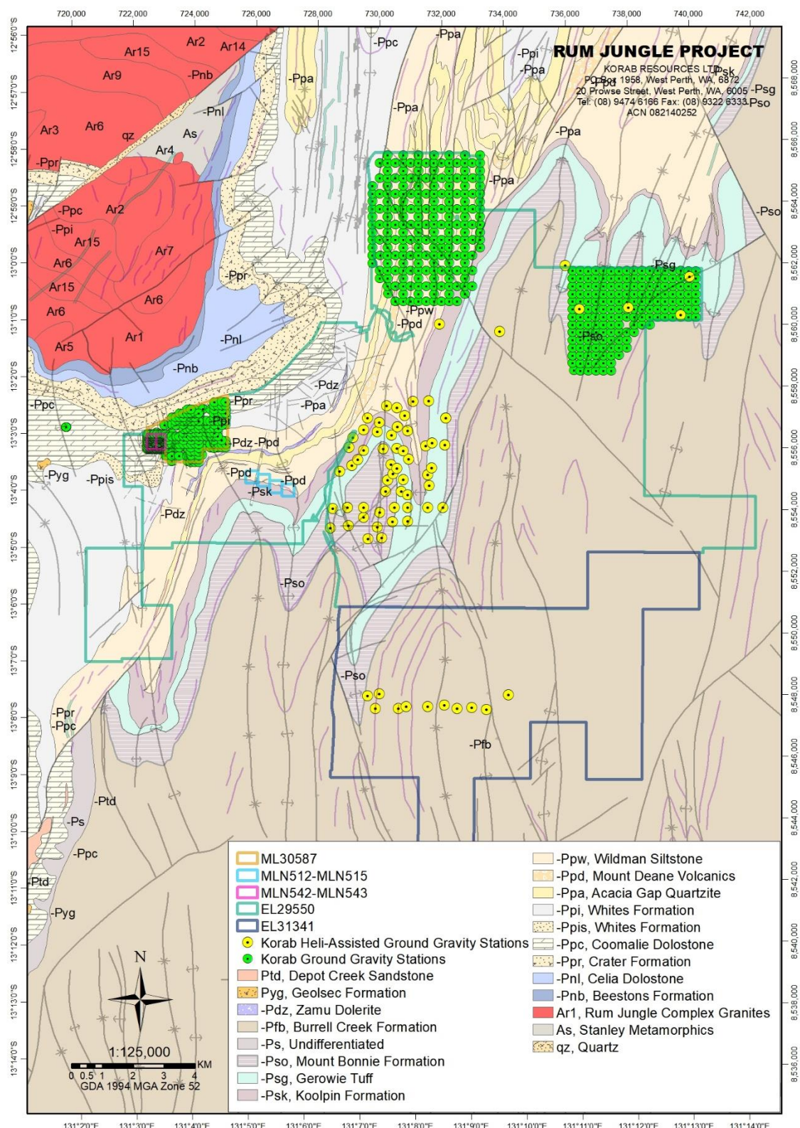
Figure 1 Completed stations of the helicopter-assisted ground gravity survey and previously reported vehicle-assisted ground gravity survey over geology and structural data
