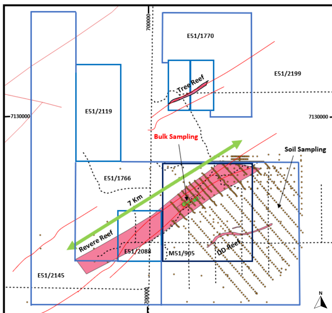
Figure 4: Revere Reef mineralised system, on tenements map
