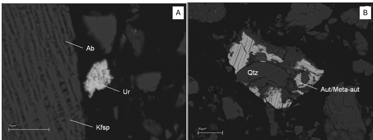
Figure 3. Backscattered electron micrograph images of Likuyu North samples. Uraninite (Ur) and autunite/meta-autunite (Aut/Meta-aut) grains and gangue minerals Albite (Ab), K-feldspar (Kfsp) and Quartz (Qtz)
