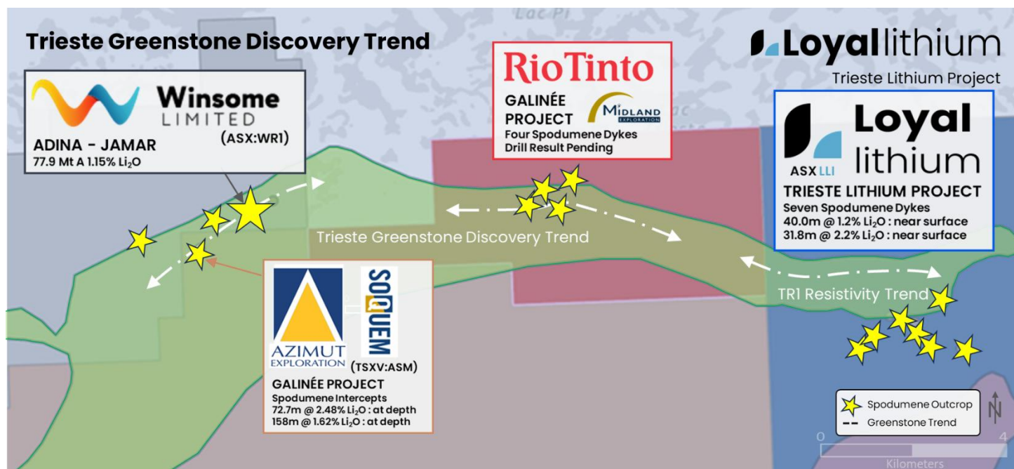
Figure 3: Trieste Greenstone Discovery Trend: Spodumene pegmatite discoveries across the Trieste Greenstone in relation to Loyal lithium's TR1 Trend and Dyke #07 discovered at the Trieste Lithium Project.
