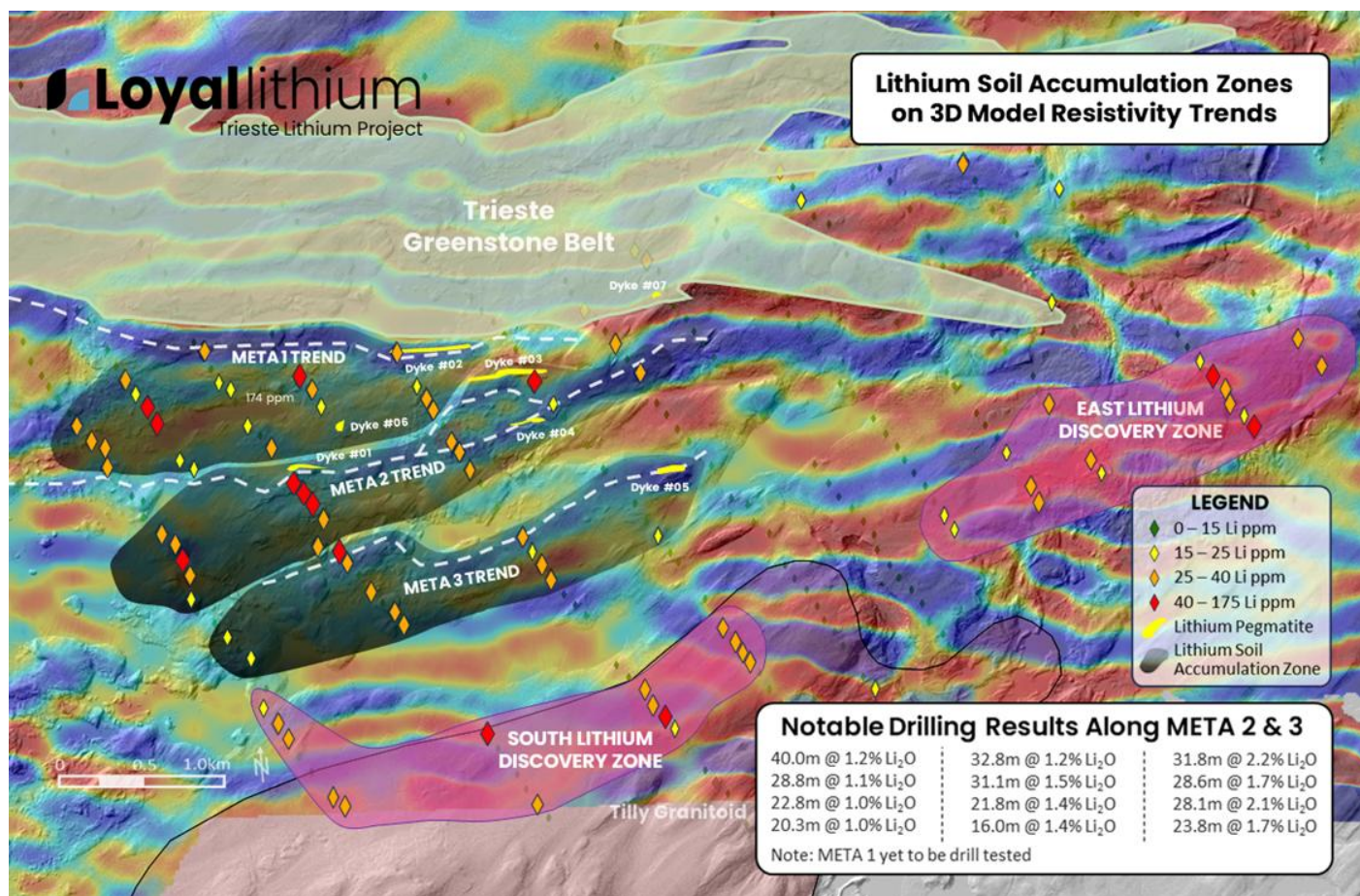
Figure 1: Trieste Lithium Project – Soil assays define Lithium Soil Accumulation Zones and two new Lithium Discovery Zones.
