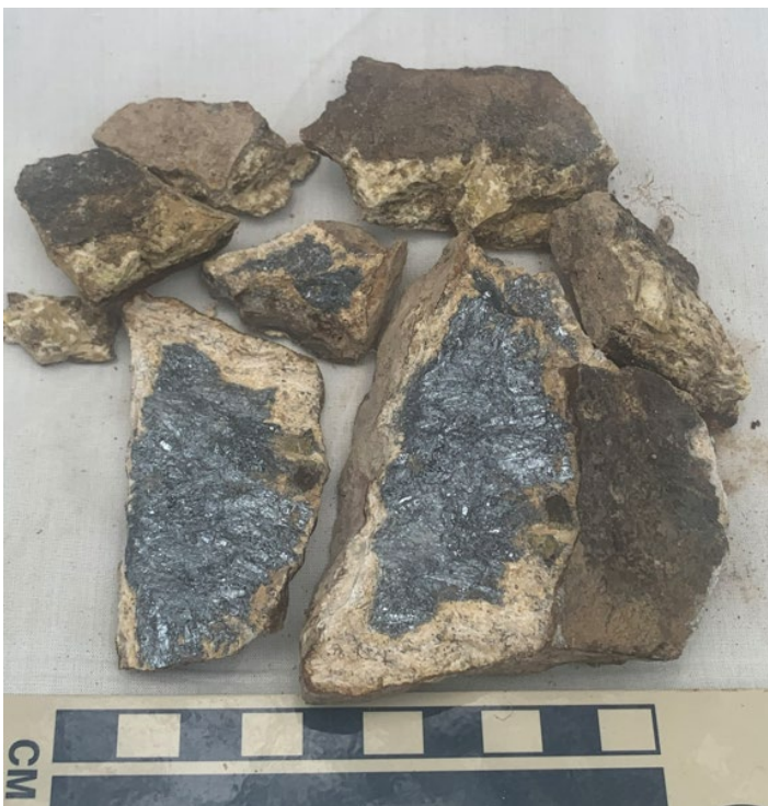
Figure 2: Left: Sample MVS16: Vein of white-lesser yellow-green antimony oxide (antimony trioxide \text{Sb}_2\text{O}_3 , 55%), and silvery-grey antimony sulphide (stibnite, \text{Sb}_2\text{S}_3 , 20%) up to 70mmx30mm, hosted in grey, silicified pelite (15%). Right: Sample MVS16: Detail of sample above, entire sample comprises vein of white-lesser yellow-green antimony oxide (antimony trioxide \text{Sb}_2\text{O}_3 , 55%), and silvery-grey antimony sulphide (stibnite, \text{Sb}_2\text{S}_3 , 20%) up to 70mmx30mm, hosted in grey, silicified pelite (25%). Note the acicular (elongate) stibnite crystals. Single rock collected from mine dump (GDA94, 56J, 6614288mN, 400905mE) and fragmented for examination (scale bar: Centimetre divisions). Sample dispatched for assay and results anticipated in 3 -4 weeks.
