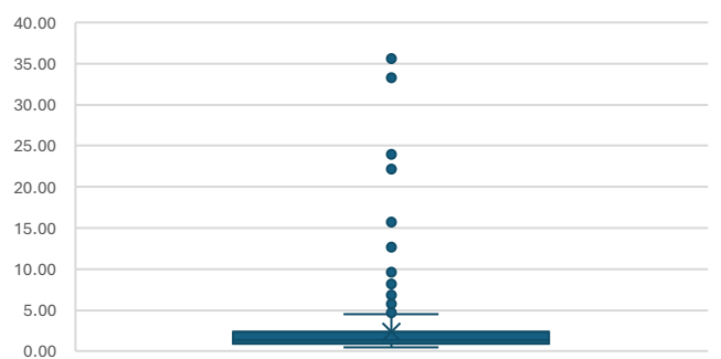
Caesium Box & Wisker Plot of all Soil Samples (ppm)
