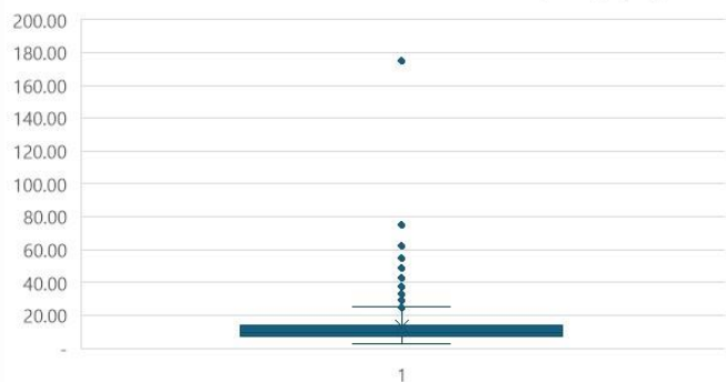
Caesium Box & Wisker Plot of all Soil Samples (ppm)
