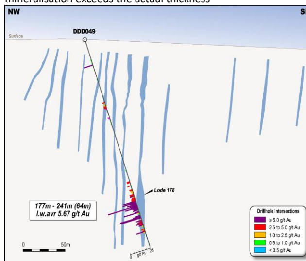
Fig. 2.6 -1 Example of the gold lodes (Cross-section looking North-East). One of the recently drilled holes (DDD049) is shown for the reference
