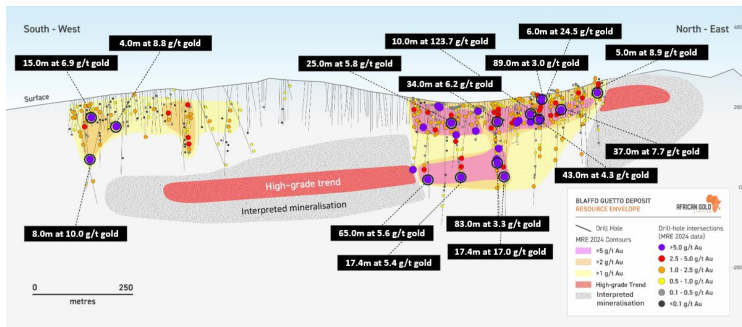
Figure 2: Blaffo Guetto MRE envelope with interpreted high grade trend and mineralisation.
