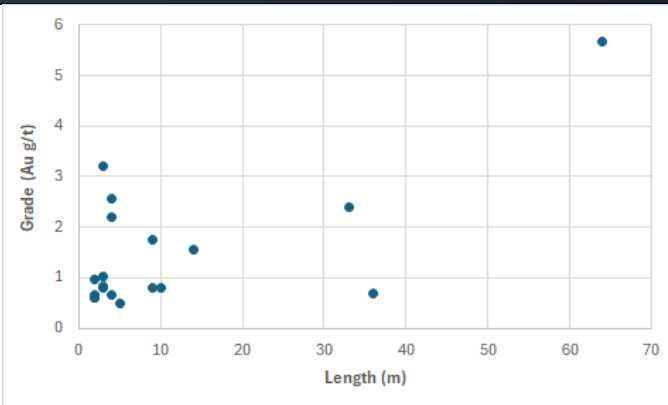
Fig. 2.5-1: Mineralised intercept
