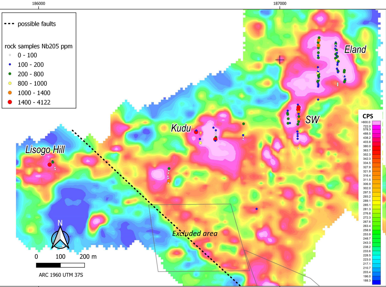
Map showing 2022 rock-chip samples over ground radiometric survey
