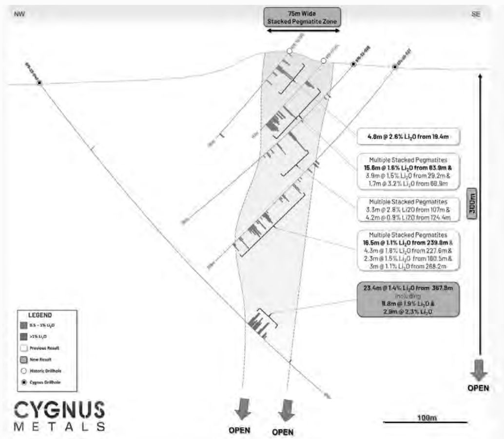
Figure 2: Cross section through Pontax Central looking towards the NE, showing both shallow historic drillholes and the recent deeper drillholes completed by Cygnus. 3 Observed geology illustrating multiple spodumene-bearing pegmatites focused over a 75m wide zone. The deepest drilling on the project to date steps out over 100m from existing drilling with mineralisation remaining open in all directions.
