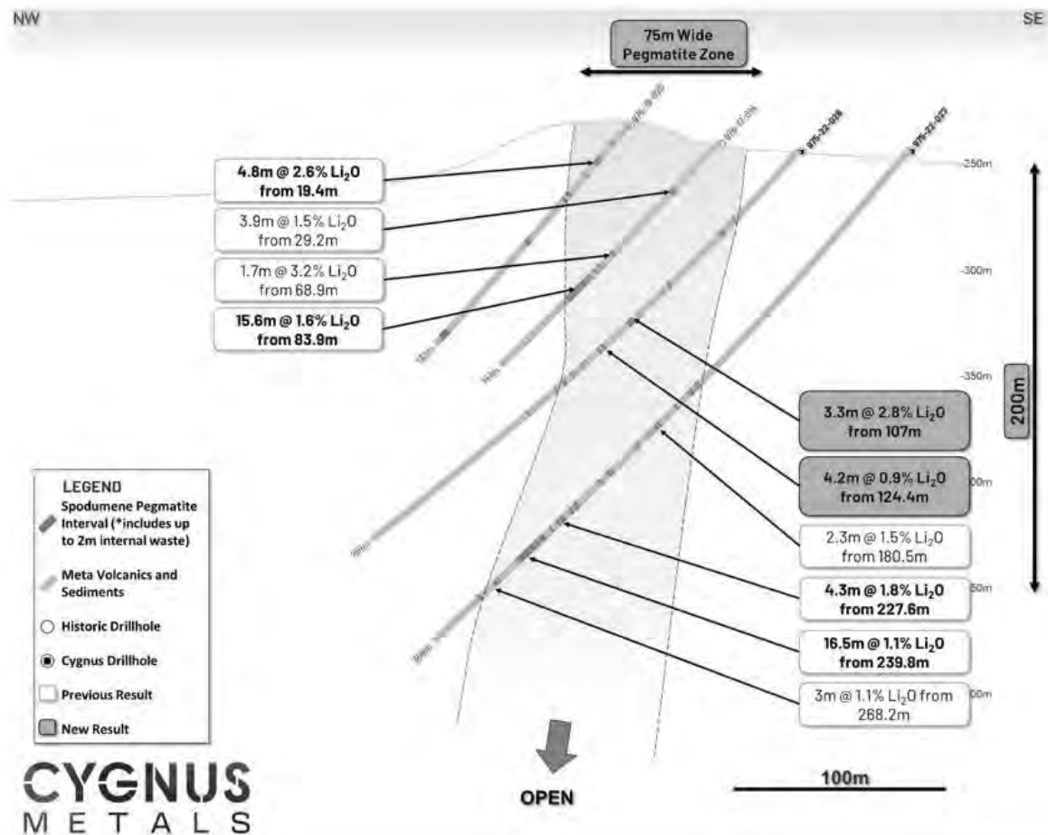
Figure 4: Cross section through Pontax Central looking towards the NE, showing both shallow historic drillholes and the recent deeper drillholes completed by Cygnus. Observed geology illustrating multiple spodumene-bearing pegmatites focussed over a 75m wide zone. The recent drilling is the deepest drilling on the project to date stepping out over 100m from existing drilling with mineralisation remaining open in all directions.
