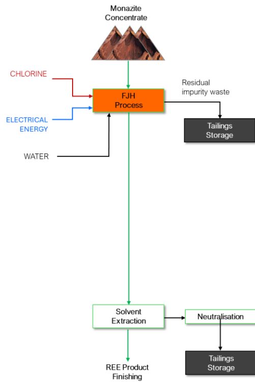
B. CONCEPTUAL FLOWSHEET USING FJH
