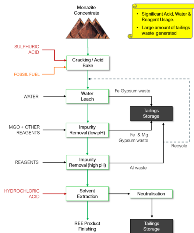
A. CONVENTIONAL FLOWSHEET FOR MONAZITE REE ORE PROCESSING
