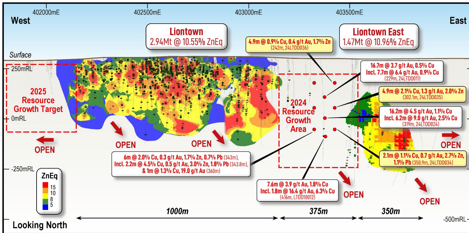
Figure 2: Long section of the ~1,600m long Lontown Resource showing the location of the recent 9 hole diamond drilling program (red dots) within the Gap Zone.
