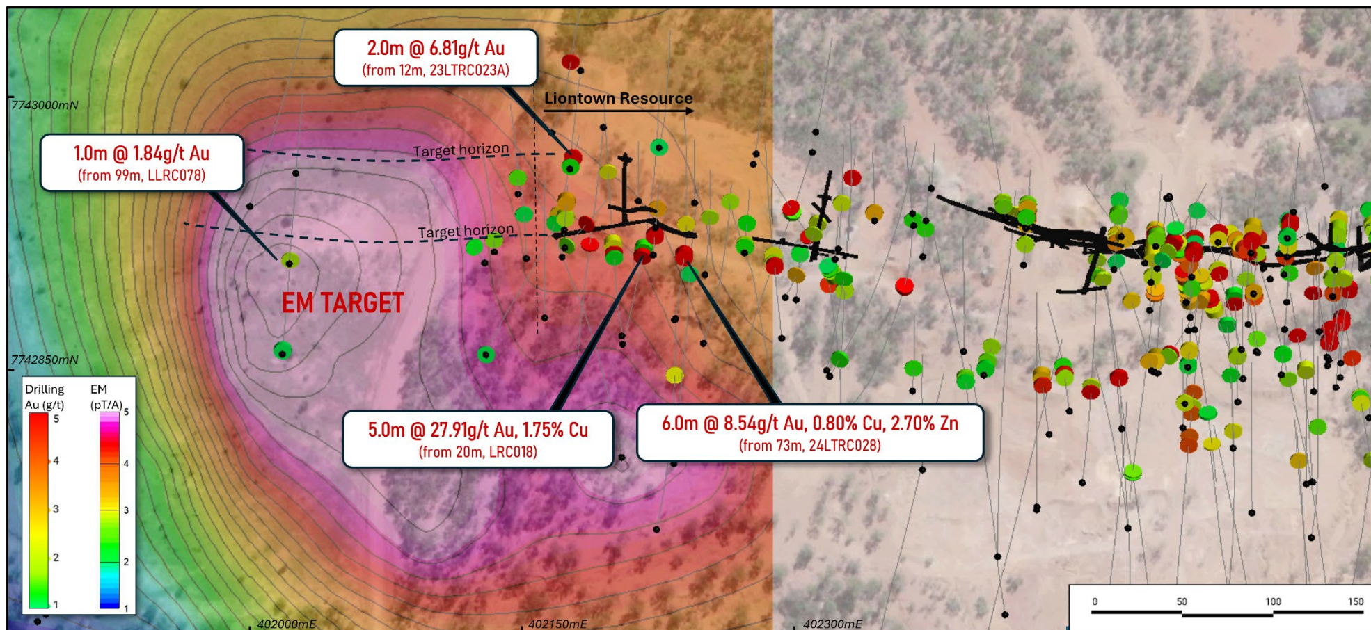
Figure 4: Plan view of the exciting Lontown West EM target showing nearby key intersections and target horizons. The target has been further validated by a “hot zone” on the western end of the Lontown Resource
