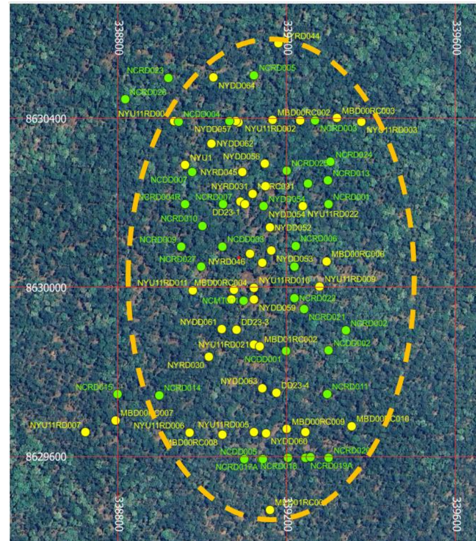
Drill collar plan for Nyungu Central showing historical holes (yellow) and Prospect holes (green) - Mineralised footprint is 1.3 km long
