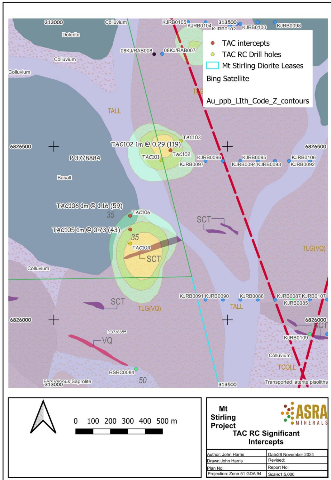
Figure 4: Diorite East RC Drill hole Significant Intercepts showing Z-score soil anomaly and underlying geological fact mapping
