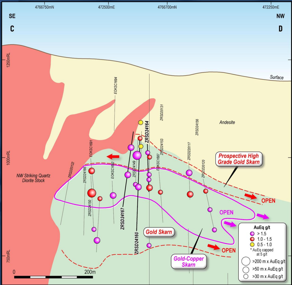
Shanac long section through the Central Domain, looking SW, 40m wide section view
