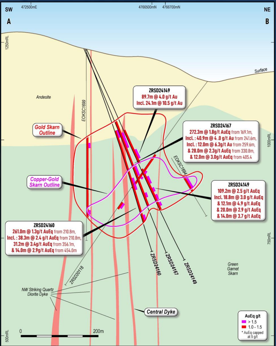
Shanac cross section looking north-west
