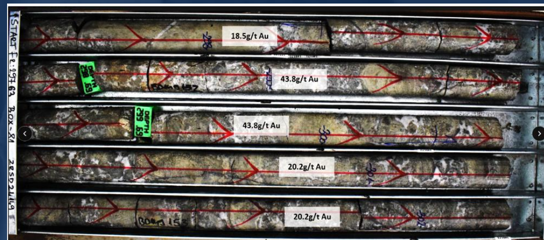
Drill core from ZRSD24149 (Shanac) 1
